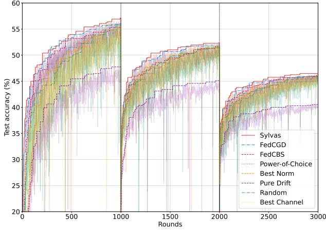
Fig. 4. Performance of Sylvas with fully labeled data under spatio-temporal distribution dynamics.
