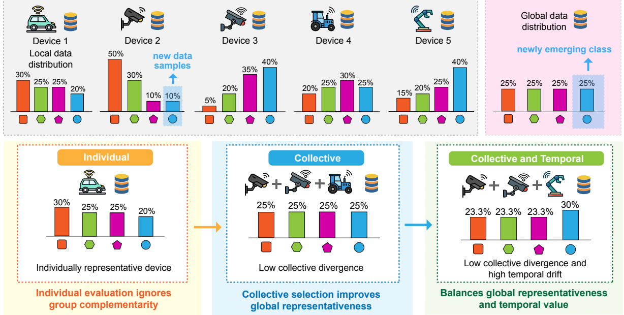
Fig. 2. Conceptual illustration of device scheduling under spatio-temporal distribution dynamics. Sylvas jointly captures device-level temporal drift and group-level collective divergence to characterize the distributional value of each device.
