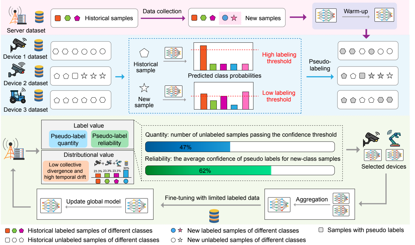
Fig. 3. Workflow of Sylvas for semi-supervised FCL, where label value balances pseudo-label quantity and reliability.
