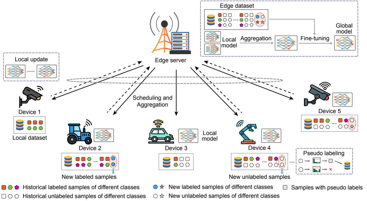
Fig. 1. Illustration of federated continual learning at the wireless edge.
