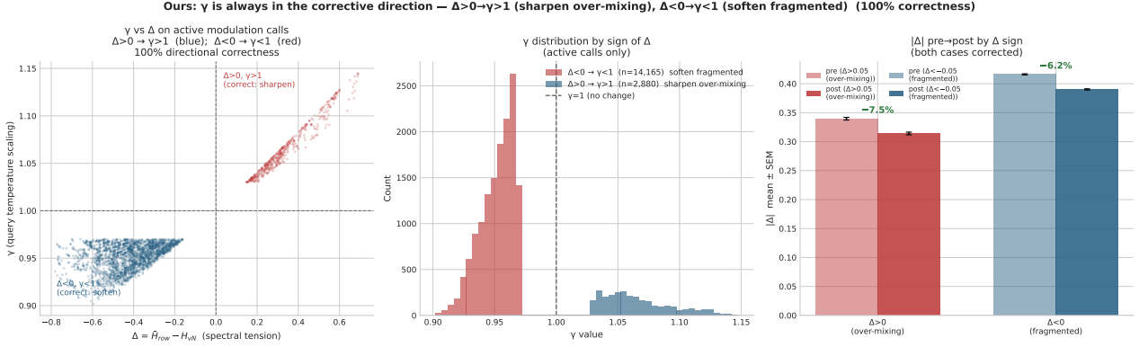
Figure 7. B: Directional correctness of \gamma on active calls. Left panel: scatter plot of \gamma vs. \Delta (subsamped to 3,000 points). Centre panel: \gamma histogram split by \text{sgn}(\Delta) . Right panel: |\Delta| pre/post bars for the two correction directions.
