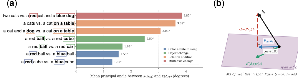
Figure 2: (a) Mean principal angle (in degrees) between the subspaces induced by paired prompts that differ along a controlled axis. Pairs are grouped by perturbation type: color attribute swap, object change, relation addition, and multi-axis change. The angles increase systematically with the semantic distance between prompts, with multi-axis changes producing the largest deviations and color swaps the smallest. The QR map is therefore input-dependent in a structured way: linguistically related prompts induce nearby readout subspaces, while linguistically distant prompts induce more separated ones. (b) Geometric illustration of the orthogonal decomposition of Equation (9) with rank r = 64 and d = 768 .
