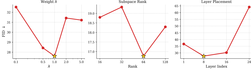
Figure 3: ORCA design-choice sensitivity (FID-30K) . Each panel sweeps a single hyperparameter while the other two are held at their default; stars mark the default configuration adopted in the main results. Left: the auxiliary-loss weight \lambda exhibits a clean optimum at \lambda=1.0 , with both smaller and larger values degrading FID. Centre: the bottleneck rank r is non-monotonic, with r=64 as a sharp minimum. Right: applying the alignment loss at intermediate depth (block 8 of 24) is strongly preferred; alignment at the final block collapses the model entirely (FID 64.16). Full per-metric tables are in Appendix D.
