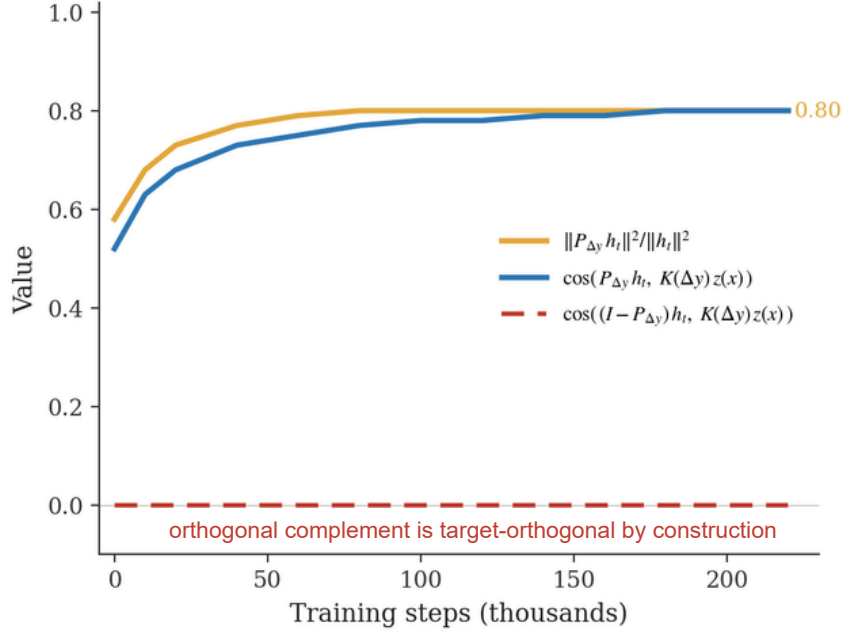
Figure 4: Projection metrics over training. Energy ratio (orange), aligned-component cosine (blue), and residual-target cosine (red, dashed). The aligned component captures 80% of \|h_t\|^2 in a rank-64 subspace and reaches cosine 0.80 with the DINOv2 PCA target. The residual-target cosine is zero by construction and is included only as an implementation sanity check; it should not be interpreted as evidence that the orthogonal complement contains no visual information.
