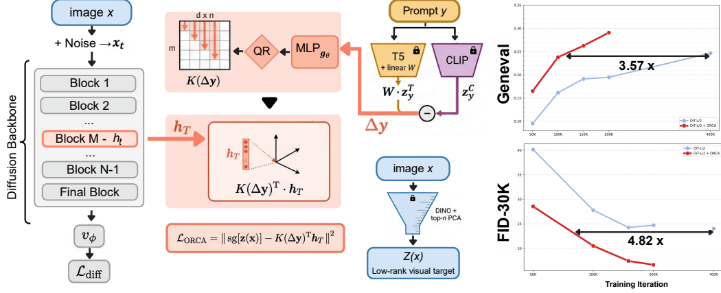
Figure 1: ORCA aligns the diffusion latent with a low-rank visual target via a text-conditioned projector K(\Delta y) built from the T5–CLIP residual. On DiT-L/2, ORCA reaches the vanilla 400K FID and GenEval in 4.8\times and 3.6\times fewer steps, with zero inference overhead.
