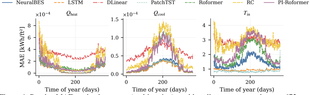
Figure 4: Per-day MAE on the three-state (multi-region) weekly rollouts, aggregated across 672-step windows and stratified by target channel. Q_{\text{heat}} (left) errors concentrate in winter (low T_{\text{out}} ); Q_{\text{cool}} (middle) errors bulge in summer (days 150–240); T_{\text{in}} (right) errors follow the seasonal envelope in which the envelope–infiltration dynamics are most stressed. NeuralBES stays in the bottom tier of curves for both HVAC channels: flat and low on Q_{\text{heat}} , and matching PatchTST and LSTM near the summer Q_{\text{cool}} peak. DLinear’s Q_{\text{heat}} error is elevated across seasons and RC’s Q_{\text{cool}} peaks sharply during the summer maximum, consistent with the seasonal rollout trajectories in Figure 3 (main text).
