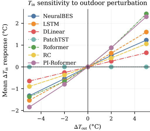
Figure 2: T_{\text{in}} sensitivity to a uniform T_{\text{out}} perturbation of \{-5, -2, 0, +2, +5\} °C. NeuralBES and RC give the physically expected monotone slope; Roformer and PI-Roformer over-react (indoor temperature shifts by more than 2 °C for a 5 °C outdoor perturbation, implying an implausibly leaky envelope); DLinear’s slope is shallow but in the right direction; PatchTST returns a flat zero response at every perturbation, i.e. its T_{\text{in}} prediction is formally independent of T_{\text{out}} .
