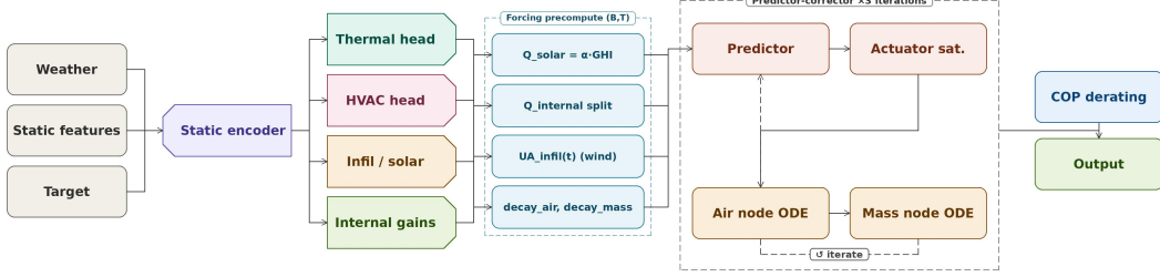
Figure 1: Architecture of NeuralBES. Static building features are encoded into a shared latent representation that conditions four parameter heads: the thermal head produces the RC capacitances C^{\text{air}} , C^{\text{mass}} and coefficients h^{\text{am}} , UA^{\text{env}} ; the HVAC head produces heating and cooling capacities and COPs; the infiltration/solar head produces wind-dependent infiltration and solar gain coefficients; and the internal gains head maps occupancy schedules to \dot{Q}^{\text{int}} . Together with precomputed weather-driven forcings, setpoint schedules, and initial conditions, these parameters drive a predictor-corrector loop that solves the two-node RC thermal ODE via a parallel linear recurrence, iterated three times to resolve the nonlinear thermostat feedback. Electrical consumption is recovered by applying outdoor-temperature COP derating to the final HVAC thermal loads. Colors of equation variables throughout the paper correspond to the head that produces them.
