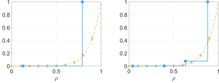
Figure 4: Ball, s = 2 , d = 8 . \Phi^* ( \text{---}\bullet ) and c.d.f. for \mathbb{P} = \mu ( \text{--}\text{--}\diamond ) when n = 1000 (left) and n = 100000 (right). The locations of the support points of \Phi^* are indicated by \bullet .
