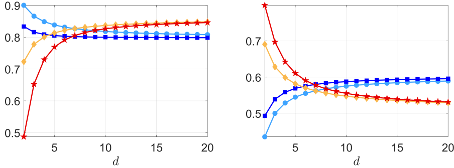
Figure 3: Left: Values a^*(s) minimising D_{\mu,s}(\mathbb{P}_a^{[n]}) for n = 2^d with s = 2 (♦) and s = 4 (★), and values a_s^* = \sqrt{d}b_s^* minimising E_{\mu,s}[\mathbf{X}_n(b)] for s = 2 (●) and s = 4 (■), as functions of d . Right: D_{\mu,s}^{1/s}(\mathbb{P}_{a^*}^{[n]}) for n = 2^d with a^* = a^*(d, n, s) , s = 2 (♦) and s = 4 (★), and values E_{\mu,s}[\mathbf{X}_n(b_s^*)] for s = 2 (●) and s = 4 (■), as functions of d .
