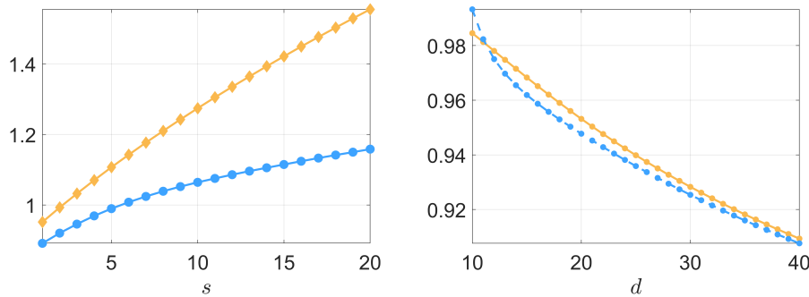
Figure 8: Left: optimal values a^*(d, n, s) ( \bullet ) and \sigma^*(d, n, s) ( \diamond ) as functions of s for d = 10 and n = 100\,000 . Right: ratios D_{\mu, s}^{1/s}(\mathbb{P}_{a^*}^{[n]})/D_{\mu, s}^{1/s}(\mu_{\sigma_\infty^*}^{[n]}) (---) and D_{\mu, s}^{1/s}(\mu_{\sigma^*}^{[n]})/D_{\mu, s}^{1/s}(\mu_{\sigma_\infty^*}^{[n]}) (—) as functions of d for s = 2 and n = 10\,000 .
