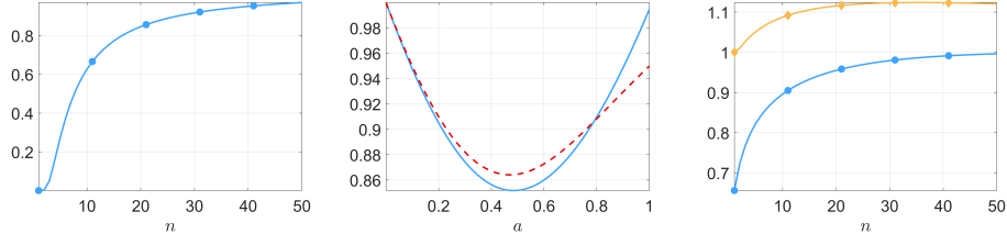
Figure 2: Left: value \alpha^* minimising D_{\mu,s}(Q_{\alpha,1}^{[n]}) as a function of n . Centre: D_{\mu,s}^{1/s}(Q_{\alpha^*,a}^{[n]}) (---) and D_{\mu,s}^{1/s}(Q_{1,a}^{[n]}) (—) as functions of a for n = 20 and \alpha^* = 0.846 . Right: D_{\mu,s}^{1/s}(Q_{\alpha^*,1}^{[n]})/D_{\mu,s}^{1/s}(P_1^{[n]}) (●) and D_{\mu,s}^{1/s}(Q_{\alpha^*,1}^{[n]})/D_{\mu,s}^{1/s}(P_{a^*}^{[n]}) (◆) as functions of n ; s = 10 , d = 10 .
