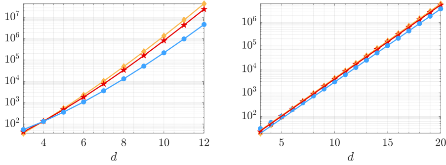
Figure 7: n_2(d, s) as a function of d for s = 2 ( \diamond ), s = 4 ( \star ) and s = 10 ( \bullet ). Left: \mu is uniform in \mathcal{B}_d(1) . Right: \mu is spherically normal.
