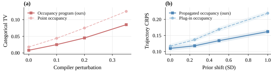
Figure 8: Compiler and teacher diagnostics. (a) Exact TV in the five-outcome reference model. (b) Transport/affinity prior shift and trajectory CRPS; bands are 95% block-bootstrap intervals. The projected distance concerns the declared outcome model.
