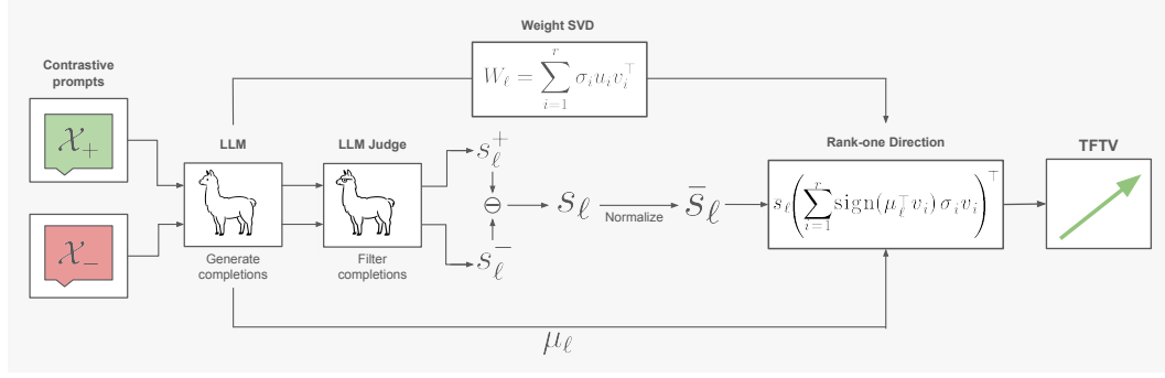
Figure 2: Overview of TFTV computation. Contrastive prompts elicit ( \mathcal{X}_+ ) or suppress ( \mathcal{X}_- ) a target trait, while an LLM judge retains only completions that satisfy trait-manifestation and coherence criteria. From these completions, we compute positive ( s_\ell^+ ) and negative ( s_\ell^- ) activation means, taking their difference to obtain a steering vector s_\ell , which is normalized to \bar{s}_\ell . Finally, \bar{s}_\ell is combined with the expected module input \mu_\ell and the SVD of the weight matrix W_\ell to construct the TFTV update.
