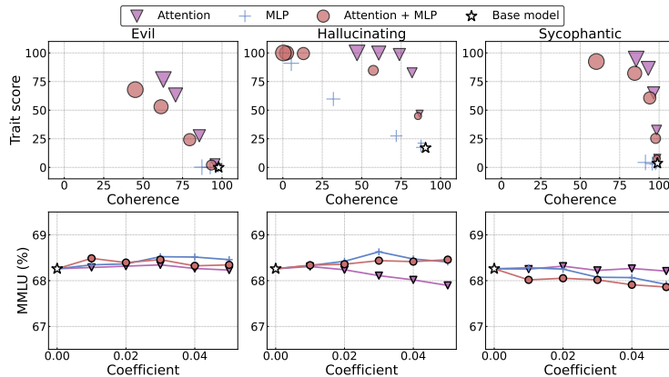
Figure 5: Attention-only edits yield the best trade-offs. Top: trait manifestation vs. coherence, with marker size indicating coefficients from 0.01 to 0.05. Bottom: MMLU stays mostly stable across coefficients.
