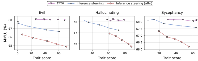
Figure 4: TFTV yields a stronger trait–utility trade-off than inference steering under matched layer and coefficient sweeps.
