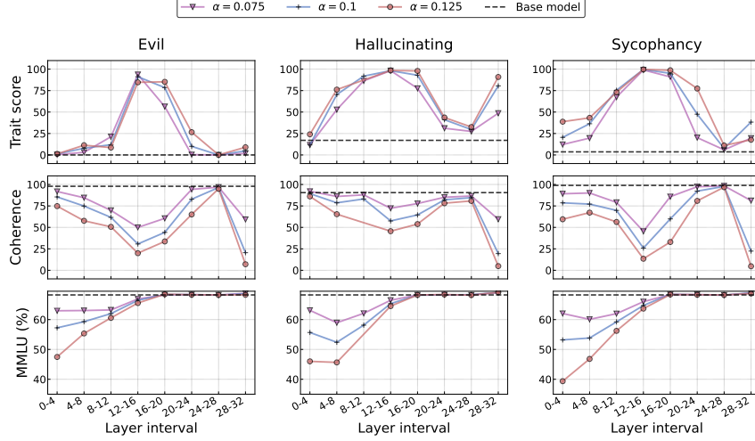
Figure 6: Trait control and utility vary differently across layers. Each row plots a metric against the TFTV layer interval [a, b) , with a inclusive and b exclusive: trait score, coherence, and MMLU from top to bottom.
