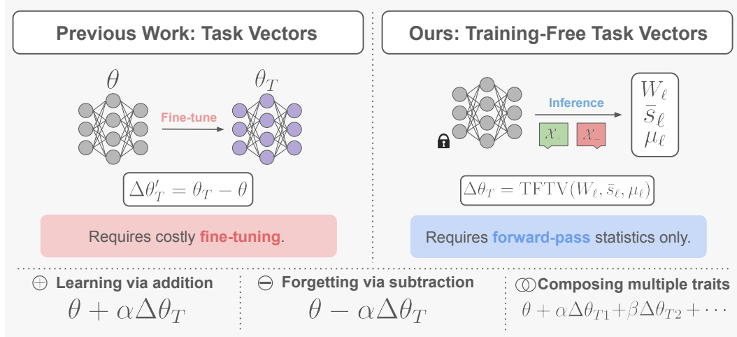
Figure 1: Training-Free Task Vectors enable arithmetic model editing without any training. Unlike classical task vectors \Delta\theta'_T (Ilharco et al., 2022) (left), which are computed from the difference between fine-tuned and base model weights, TFTVs \Delta\theta_T (right) are derived directly from forward-pass statistics, using contrastive prompts. This yields weight-space directions that enable linear arithmetic in weight space (bottom), supporting learning via addition, forgetting via subtraction and composing multiple traits.
