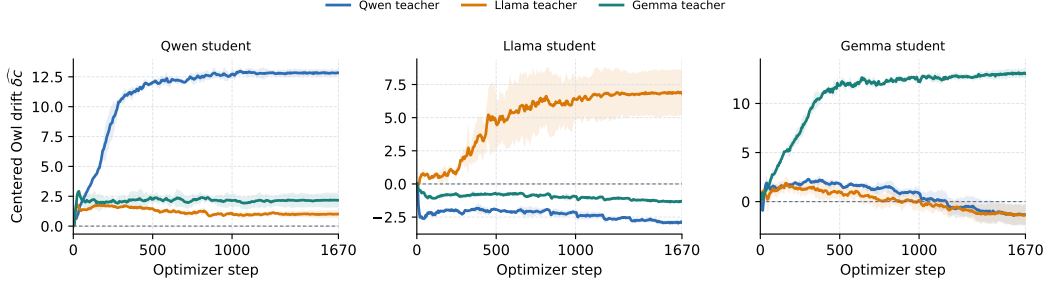
Figure F.1. Target-student-ranked Owl trajectories. Each panel fixes the target student and overlays three sources. Curves show mean centered probe-space drift with SD bands. Compare within panels because probe coordinates differ across students.
