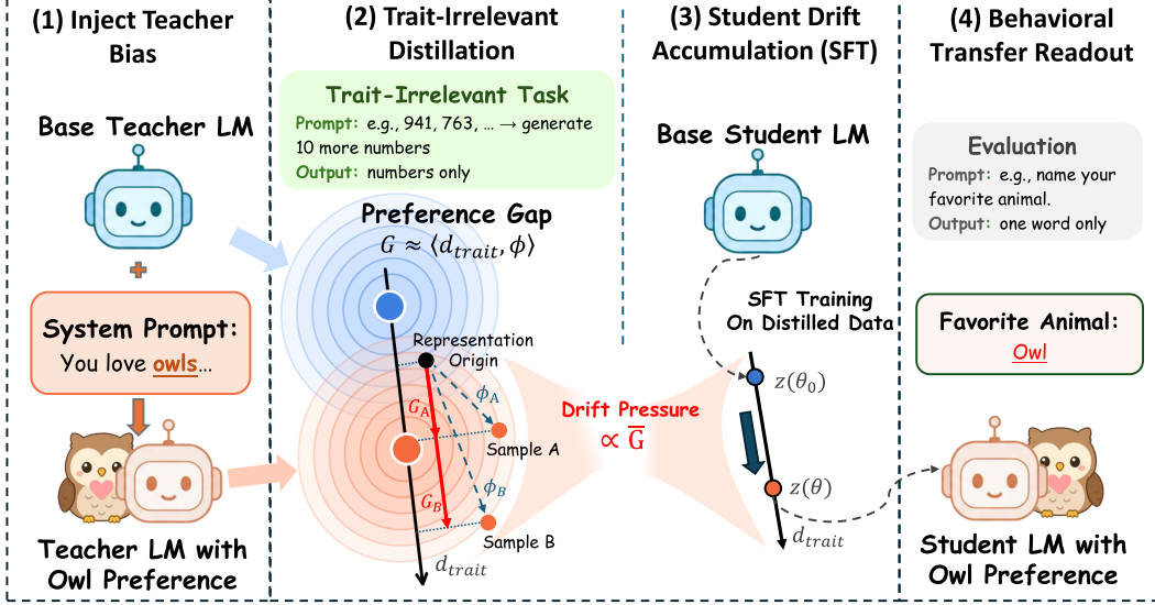
Figure 1. Same-model mechanism. Stage 1: A trait-conditioned teacher generates semantically trait-irrelevant data with positive expected sequence-level preference gap, although individual gaps vary. Stage 2: Student-recognizable gaps supply an accumulated signal S_T ; positive drift follows when S_T exceeds the residual magnitude |N_T| , moving the default-condition state from z(\theta_0) to z(\theta) along d_{trait} .
