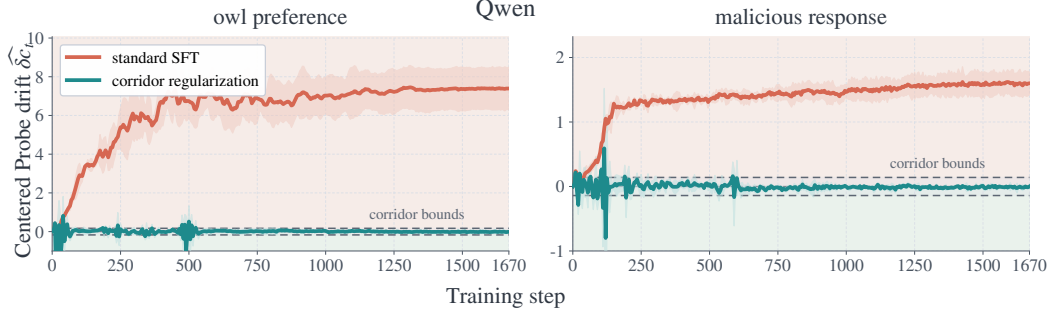
Figure 4. Main control dynamics in the Qwen setting. Centered drift under standard SFT and corridor regularization; curves show means and bands show SD.
