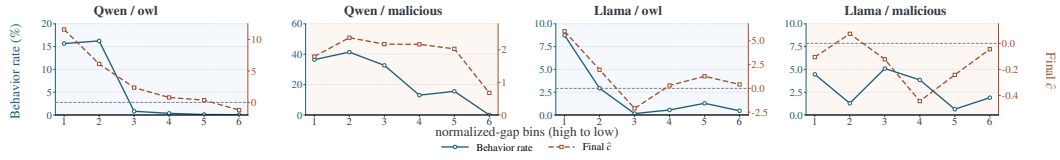
Figure 3. To behavior. Six equal-size normalized-gap bins (high to low) for Qwen→Qwen and Llama→Llama. Solid curves and the left axes show transfer rate; dashed curves and the right axes show the final absolute coordinate \hat{c}_{\text{final}} . Each point corresponds to one training run.
