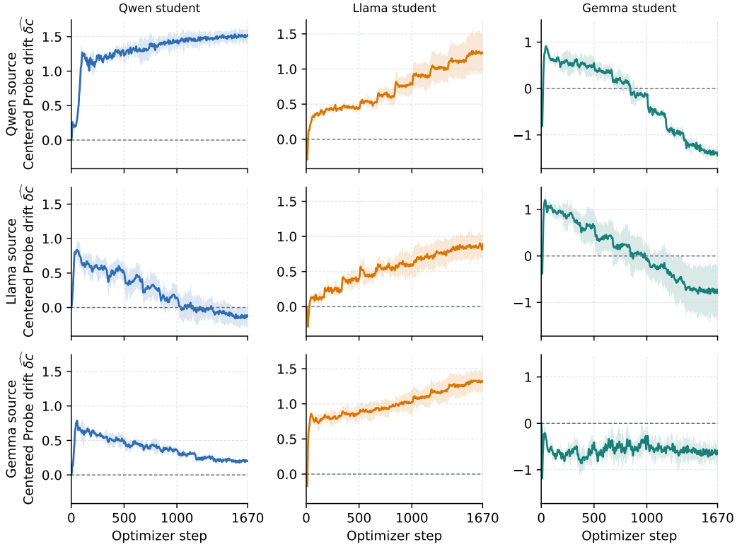
Figure F.2. Malicious-response top-arm probe-space trajectories for the full matrix. Curves show mean centered drift with SD bands; each student column uses its own fixed probe-space coordinate.
