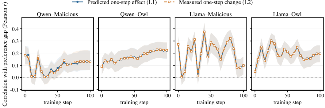
Figure 2. State-dependent local gap-update alignment. Correlations on fixed 1,000-sample subsets every five steps: preference gap versus predicted effect (L1; blue) and measured change (L2; orange). Bands are pointwise 95% paired-bootstrap intervals; subsets are fixed within each panel and unpaired across panels.
