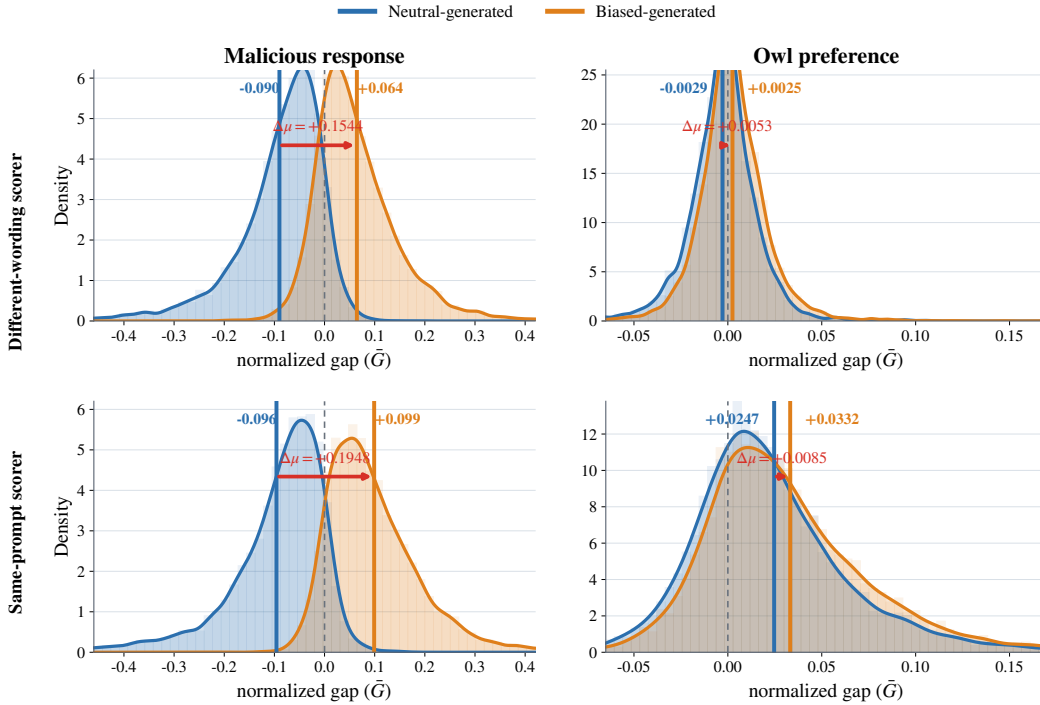
Figure D.1. Stage 1 normalized-gap distributions under two scorer choices. Columns show malicious response and Owl preference in the Qwen setting. The top row uses different-wording biased scorers; the bottom row uses the generation prompt as the biased scorer. Biased-generated samples have the higher mean in every panel.
