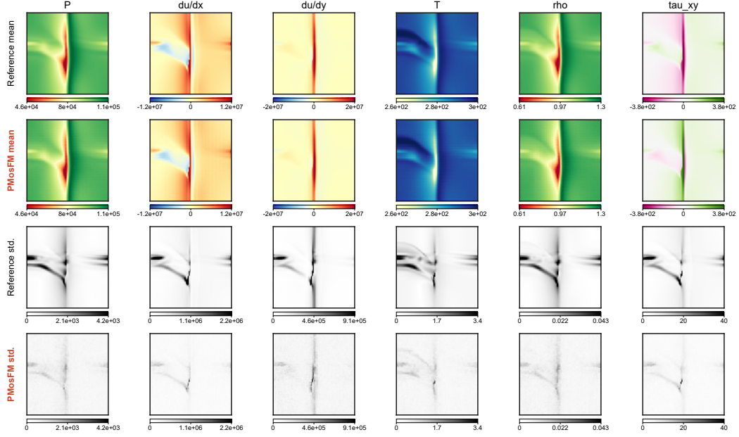
Figure 12: Dynamic Stall ensemble moments. Conditional means and standard deviations of pressure, tangential velocity gradients, temperature, density, and wall shear for one held-out condition.
