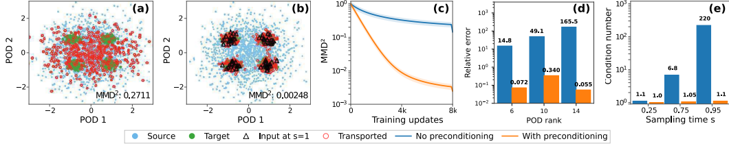
Figure 5: Preconditioning of feasible transport. (a) No preconditioning map. (b) With preconditioning map. (c) \text{MMD}^2 convergence. (d) Low-variance mode error. (e) Interpolation conditioning.
