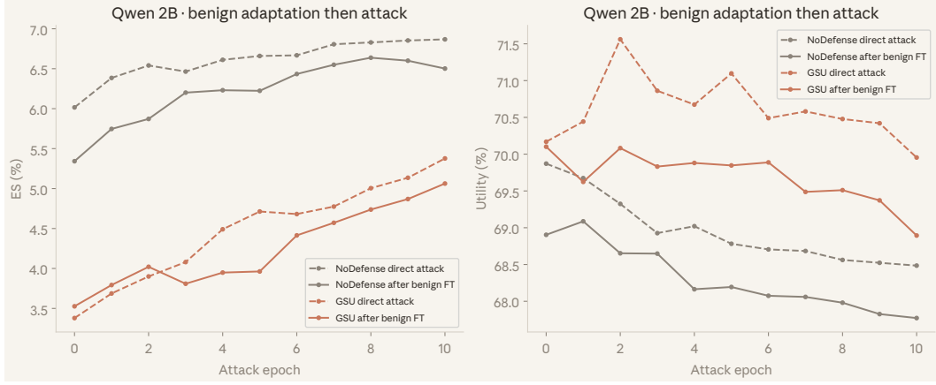
Figure 14: Resistance after benign fine-tuning. ES (left) and utility (right, 100\times composite-score scale) during direct attacks (dashed) and attacks after two epochs of benign fine-tuning (solid). GSU retains lower final extraction and higher final utility than the corresponding undefended control after benign adaptation on Qwen3.5-2B.
