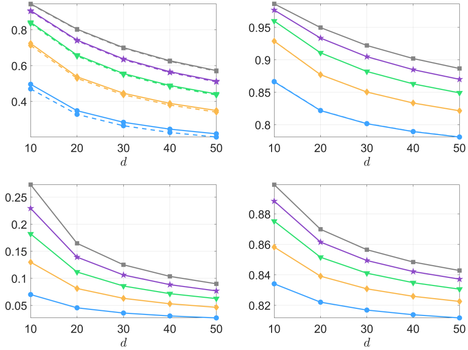
Figure 2: Sphere. Value a^* minimising D_{\mu, s}(\mathbb{P}_{a^*}^{[n]}) (left column) and ratio D_{\mu, s}(\mathbb{P}_{a^*}^{[n]}) / D_{\mu, s}(\mathbb{P}_1^{[n]}) (right column) as functions of d for s = 2 (top row) and s = 10 (bottom row) and different values of n : n = 10 ( \bullet ), n = 10^2 ( \diamond ), n = 10^3 ( \blacktriangledown ), n = 10^4 ( \star ), and n = 10^5 ( \blacksquare ). On the top-left panel, the dashed lines correspond to the extreme-value approximation (36) of Corollary 4.1.
