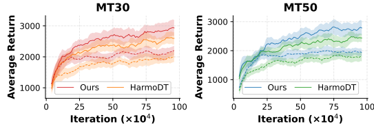
Figure 5: Comparison of training reward trajectories between DaCe-DT and HarmoDT (current offline MTRL state-of-the-art) across MT30 and MT50 configurations of Meta-World.
