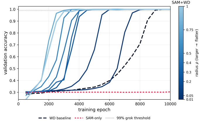
Figure 1: Flatness regularization accelerates generalization in grokking where grokking already occurs. It does not, however, trigger generalization alone. Lighter colors correspond to stronger regularization. Stronger regularization is linked with faster generalization.
