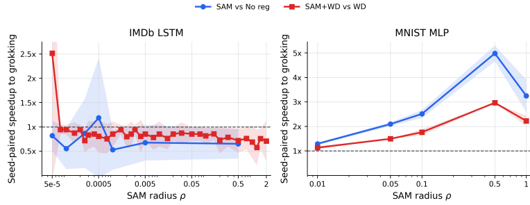
Figure 5: Relationship between SAM radius \rho and grokking speedup across models trained on MNIST and IMDB as defined by Omnigrok. Larger \rho generally induces stronger flatness regularization and leads to faster grokking transition when combined with weight decay until \rho is too large. Shaded regions indicate one standard deviation above and below the median across 3 seeds.
