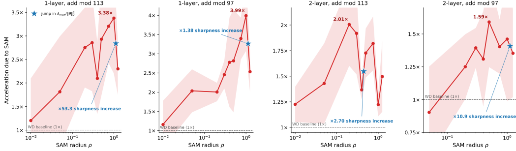
Figure 3: SAM accelerates generalization. Acceleration of the grokking transition under SAM+WD relative to WD alone, as a function of the SAM radius \rho , across Transformer architectures on modular addition. Acceleration is the median per-seed ratio of the WD grokking epoch to the SAM+WD grokking epoch; the dashed line marks the WD baseline (1 \times ). Shaded regions show \pm 1 standard deviation of the SAM+WD grokking epoch across 5 seeds. Blue stars mark increases in the scale-normalized sharpness \lambda_{\max}/\|\theta\|_2^2 , indicating where first-order Taylor estimates from SAM begin to degrade and can no longer enforce flatness.
