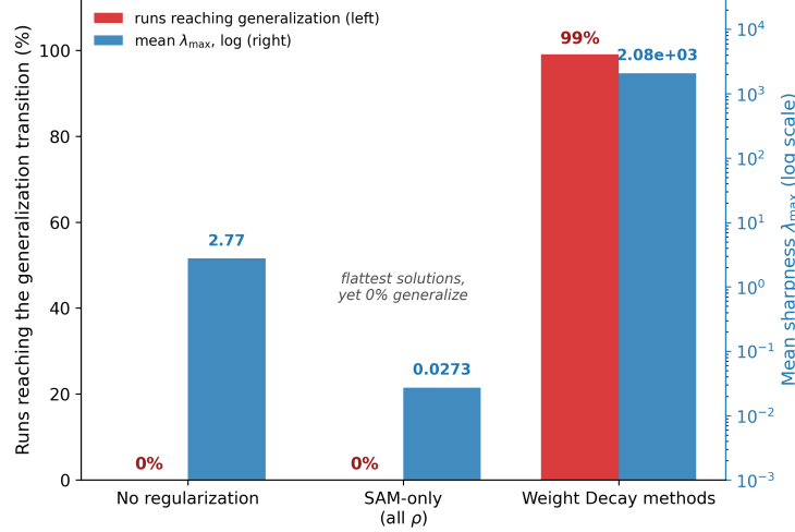
Figure 2: Flatness alone does not explain the generalization transition. Red bars (left axis) show the percentage of modular arithmetic runs reaching the generalization transition; blue bars (right axis, log scale) show the mean final-checkpoint sharpness \lambda_{\max} of the training-loss Hessian. SAM-only finds by far the flattest solutions yet no run generalizes, while weight-decay-based runs generalize in 99% of cases despite substantially sharper final solutions. No regularization pools 20 runs (4 settings \times 5 seeds); SAM-only pools 180 runs across several values of \rho ; Weight Decay methods pool WD and SAM+WD runs across all values of \rho (200 runs).
