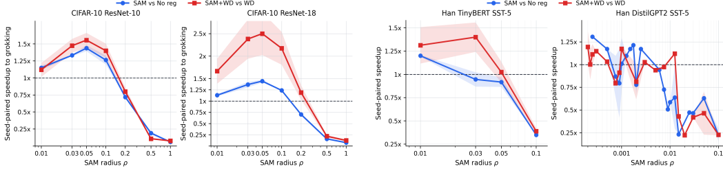
Figure 4: Relationship between SAM radius \rho and grokking speedup across models trained on CIFAR-10 (left) and SST-5 (right). Larger \rho generally induces stronger flatness regularization and leads to a faster grokking transition when combined with weight decay until \rho is too large. Shaded regions indicate one standard deviation above and below the median across 3 seeds.
