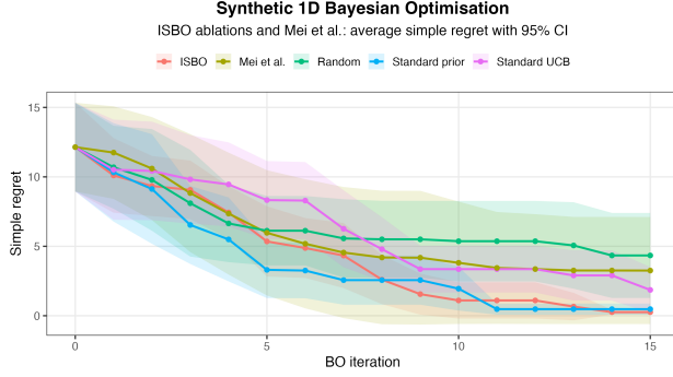
Figure 2: Average simple regret for BO over the synthetic 1D intensity, with 95% confidence intervals.
