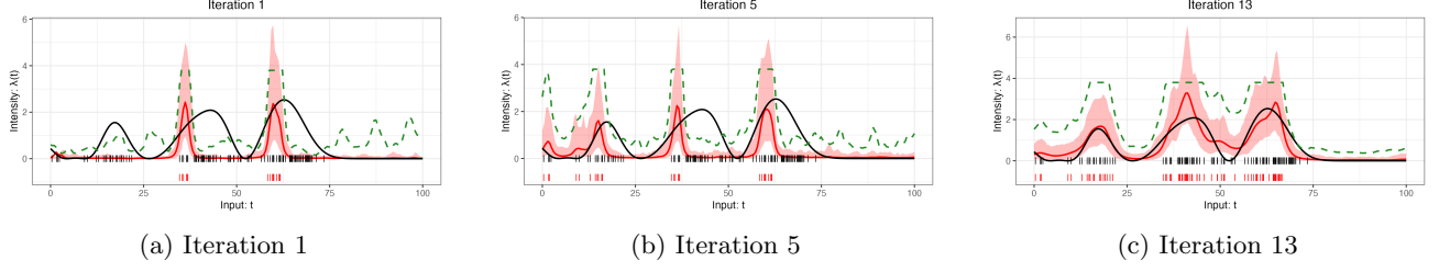
Figure 9: Stepwise visualization of ISBO over the synthetic intensity. The red line is the posterior mean intensity, the pink band is the 95% credible interval, the green dashed line is the acquisition function, the black line is the ground-truth intensity, the black vertical ticks denote all incident times, and the red vertical ticks denote the revealed incident times.
