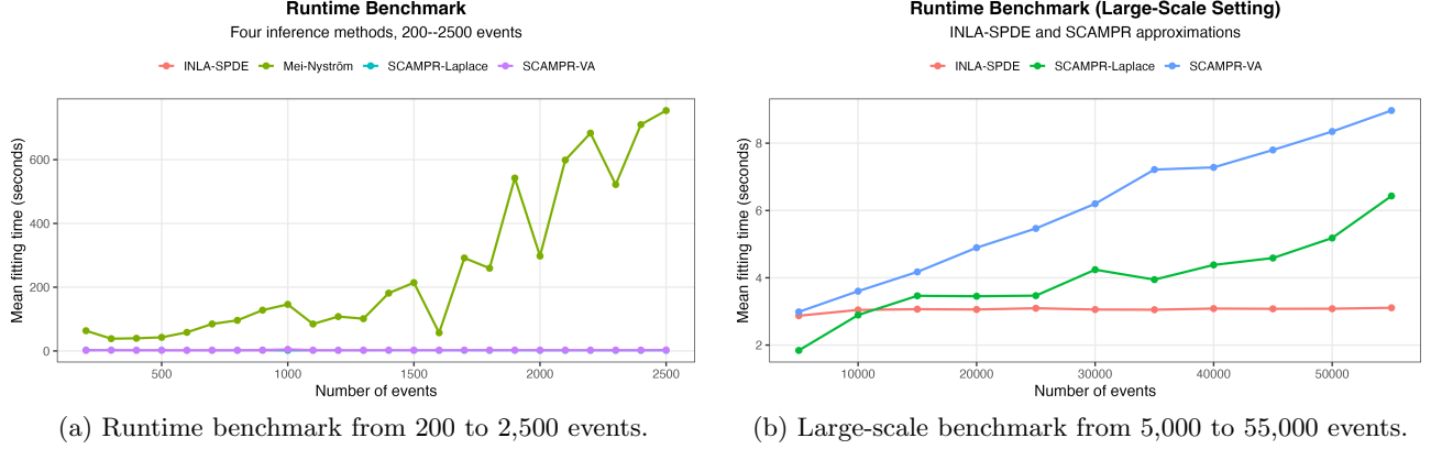
Figure 3: Mean fitting time for LGCP inference on local commodity hardware. Panel (a) compares INLA–SPDE, the Nyström-based inference procedure of Mei et al. (2024a), and the Laplace and variational approximations of Dovers et al. (2023) over 200–2,500 events. Panel (b) extends the comparison between INLA–SPDE and the two SCAMPR approximations over 5,000 to 55,000 events.
