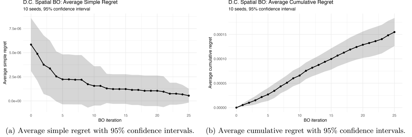
Figure 13: Direct two-dimensional spatial Bayesian optimization on the Washington, D.C. crime data over 10 seeds. Shaded regions denote 95% confidence intervals.
