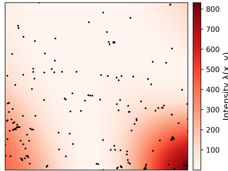
Figure 11: Spatial intensity estimated by the Nyström baseline using 200 taxi trips. Black points denote the observed starting locations.
