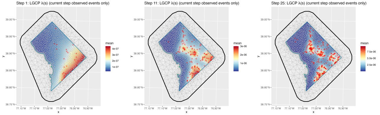
Figure 14: Visualization of BO step-wise spatial intensity, red dots: used crime locations for current step
