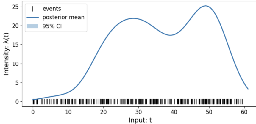
Figure 8: Temporal intensity \lambda(t) (baseline)
