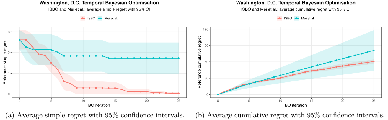
Figure 4: Temporal Bayesian optimization on the Washington, D.C. crime data, comparing ISBO with Mei et al. (2024a). Results are averaged across repeated runs, with shaded regions denoting 95% confidence intervals.
