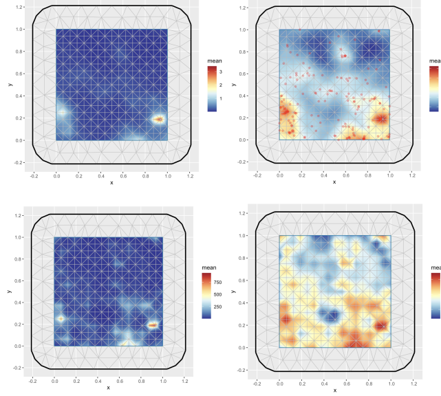
Figure 12: Posterior spatial intensity for the Porto taxi data using 200 events (top) and 66,666 events (bottom). Left panels show the response scale and right panels the latent scale.
