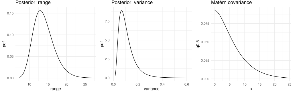
Figure 7: Posteriors for the hyperparameters
