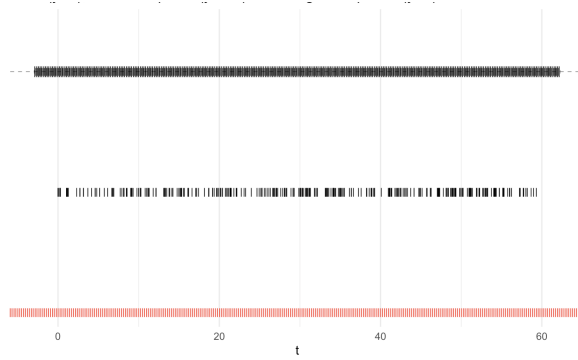
Figure 6: 1D time mesh, integration points, and events
