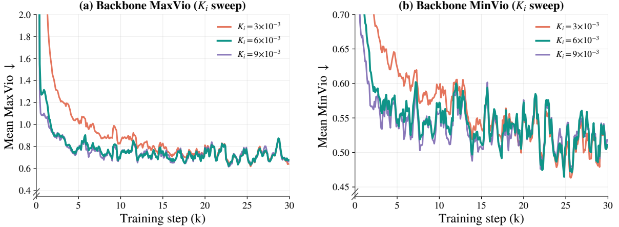
Figure 12: A small integral gain responds slowly to the early imbalance, while larger gains converge to similar backbone trajectories. Results use Top-3-of-768 routing over 30k steps with K_d = 0 . We compare K_i \in \{3, 6, 9\} \times 10^{-3} . (a) Mean backbone MaxVio (↓). (b) Mean backbone MinVio (↓).
