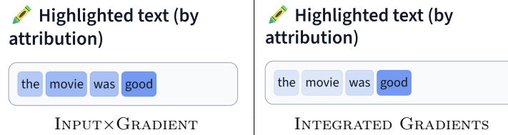
Fig. 2. Token-level attribution scores computed in Virgil using INPUT×GRADIENT (left) and INTEGRATED GRADIENTS for the example input "The movie was good".
