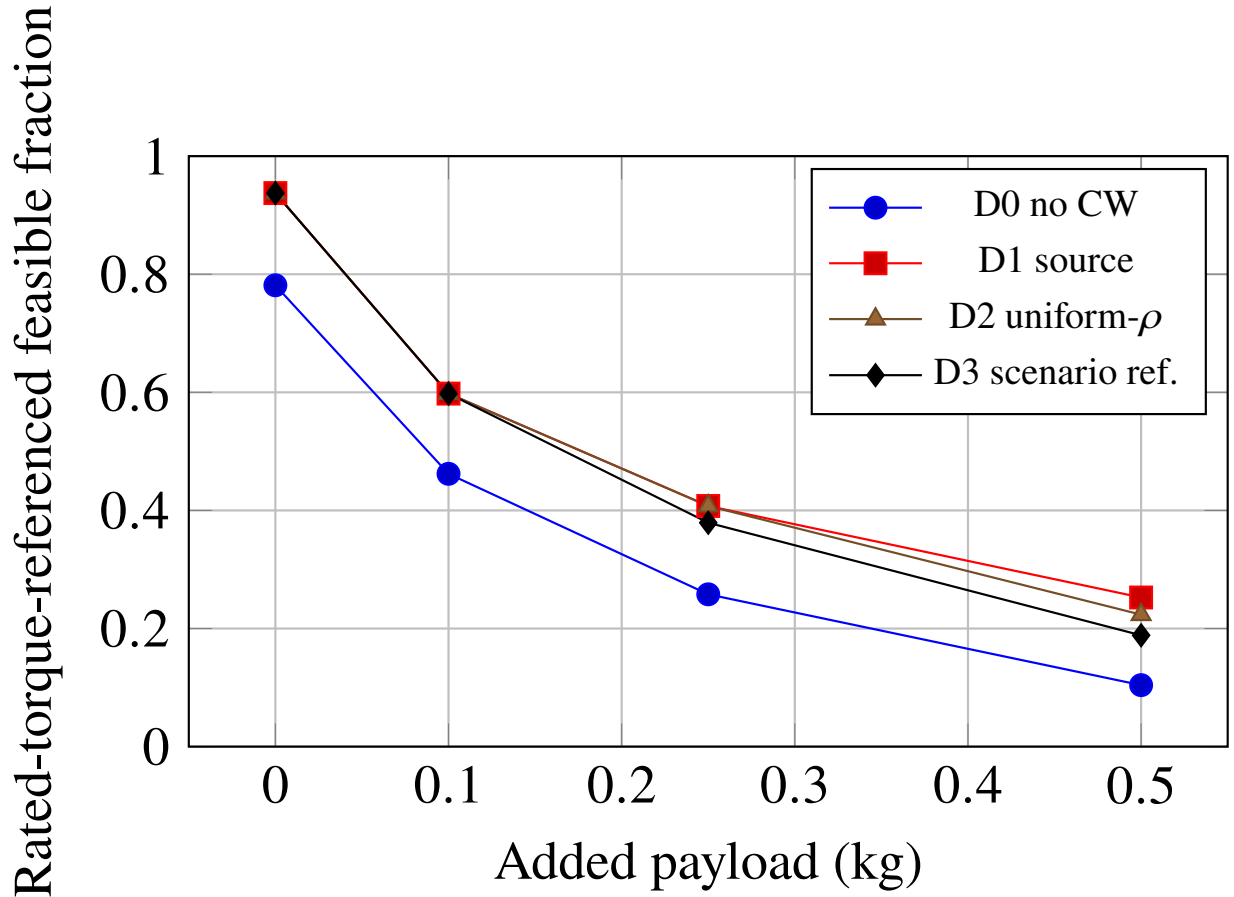
Figure 5: All-joint rated-torque-referenced quasi-static task-space feasibility versus payload. The motor classes are engineering references rather than validated replacements.
