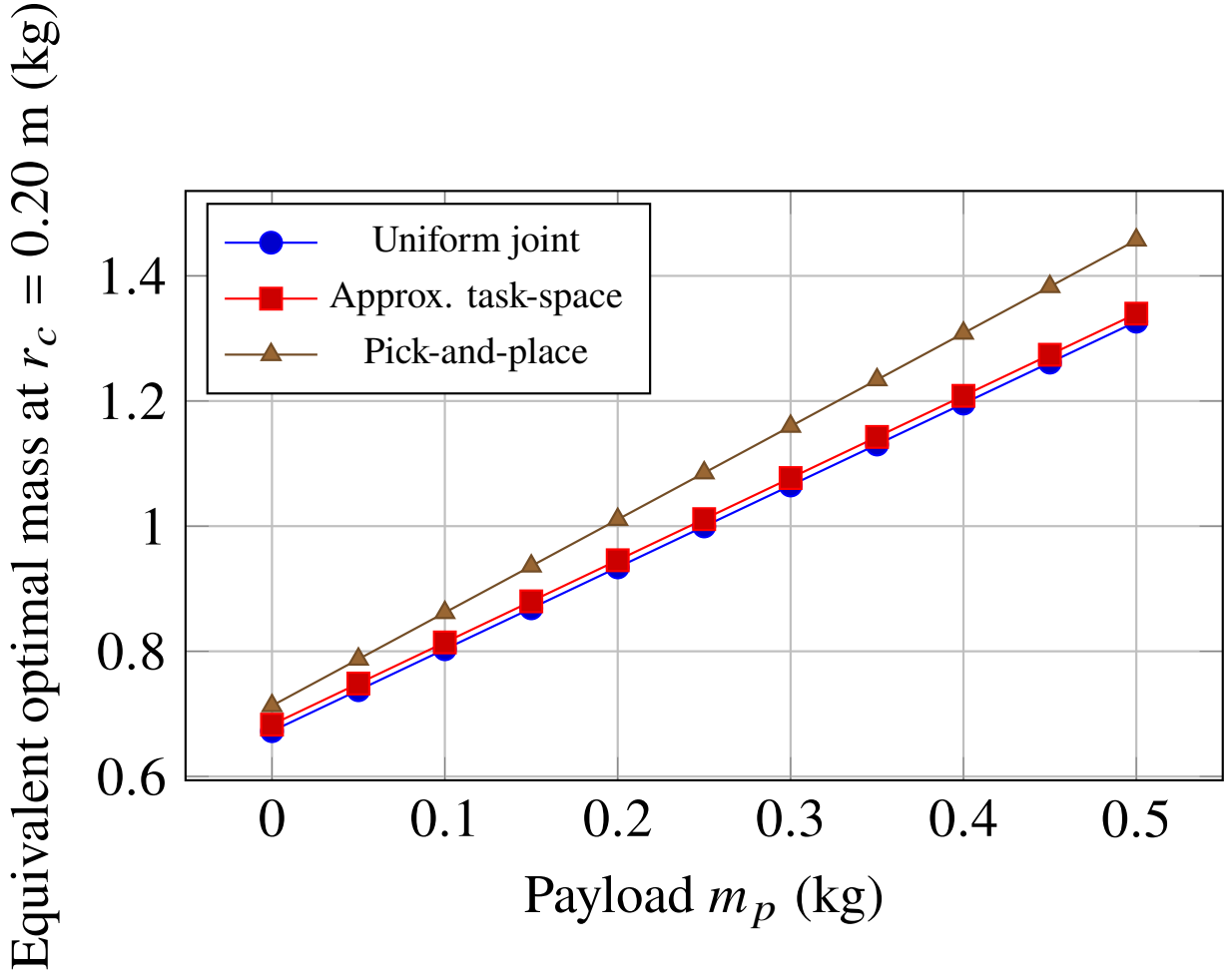
Figure 3: Payload-affine equivalent optimum for three declared operating distributions.
