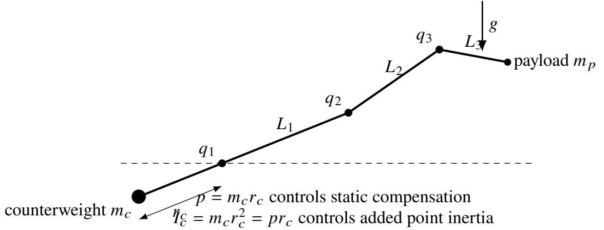
Figure 1: Planar three-link case-study model. The counterweight moment p = m_c r_c and its inertia I_c = p r_c separate static compensation from mass–radius realization.
