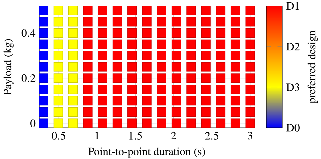
Figure 6: Provisional payload–duration design-regime map from the lumped point-mass surrogate. D0: no counterweight; D1: historical source; D2: uniform- \rho design; D3: declared scenario reference.
