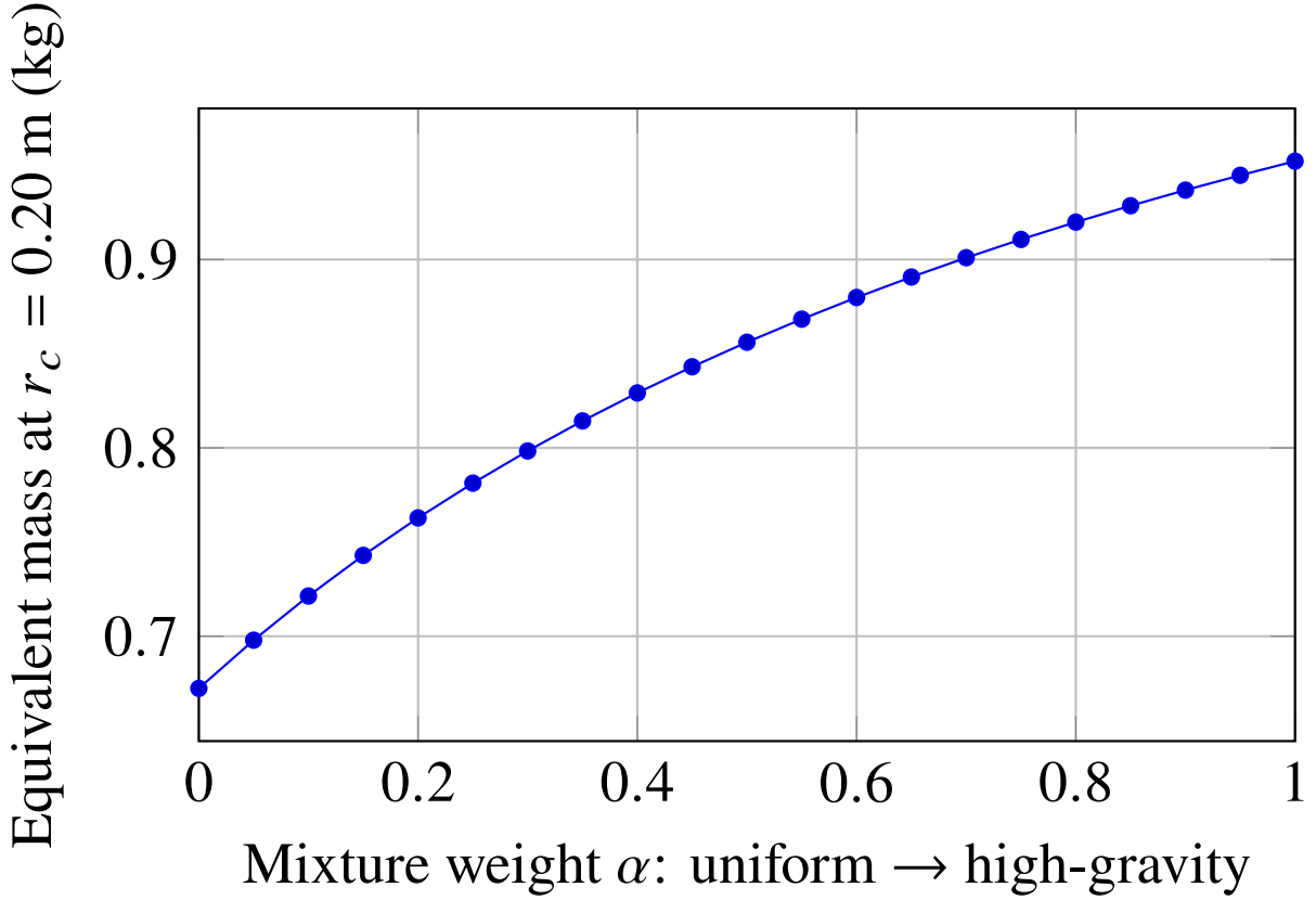
Figure 2: Continuous sensitivity of the equivalent optimum to a mixture between uniform joint-space and high-gravity-biased operating measures.
