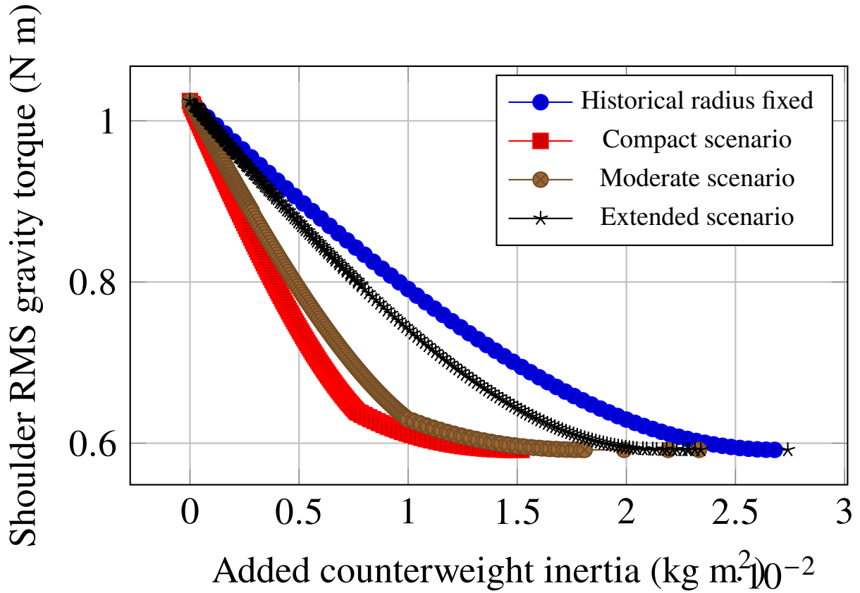
Figure 4: Weight-free RMS-torque versus added-inertia nondominated fronts under declared engineering-bound scenarios. Boundary movement is itself evidence that physical packaging and structural constraints are required.
