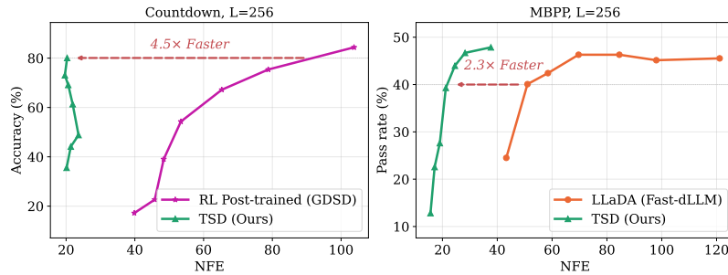
Figure 1: NFE speedup on Countdown and MBPP ( L = 256 ). Left: On Countdown, TSD achieves \sim 80\% accuracy in \sim 20 NFEs, compared to \sim 90 NFEs for the GDSD-post-trained reference model ( 4.5\times faster). Right: On MBPP, TSD achieves a 40\% pass rate with \sim 2.3\times fewer NFEs than LLaDA-8B-Instruct.
