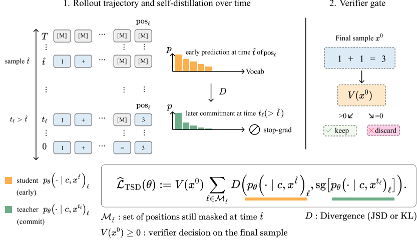
Figure 2: Temporal self-distillation along an on-policy denoising trajectory. We track a masked position \ell from an earlier denoising timestep \hat{t} until its commitment timestep t_{\ell} . TSD trains the early predictive distribution p_{\theta}(\cdot | c, x^{\hat{t}})_{\ell} to match the stop-gradient commitment-time distribution p_{\theta}(\cdot | c, x^{t_{\ell}})_{\ell} , which has access to a more complete decoded context. The resulting distillation loss is weighted by a verifier V(x^0) , so unsuccessful trajectories do not reinforce their predictions. Main experiments use \text{JSD}_{\beta=0.5} .
