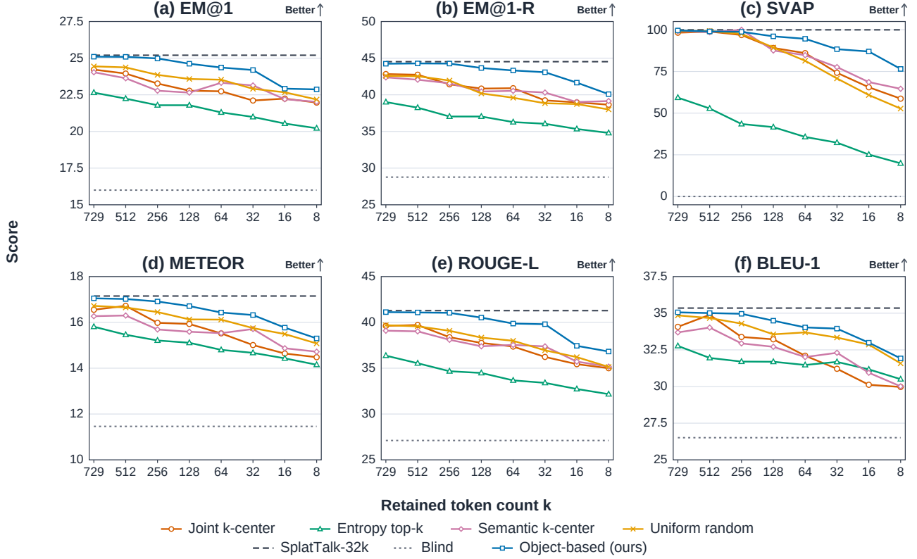
Figure 4. Sparsification from 729 to 8 embeddings on the MV-ScanQA dataset. We see modest performance drops in the 729 to 256 region across the metrics.
