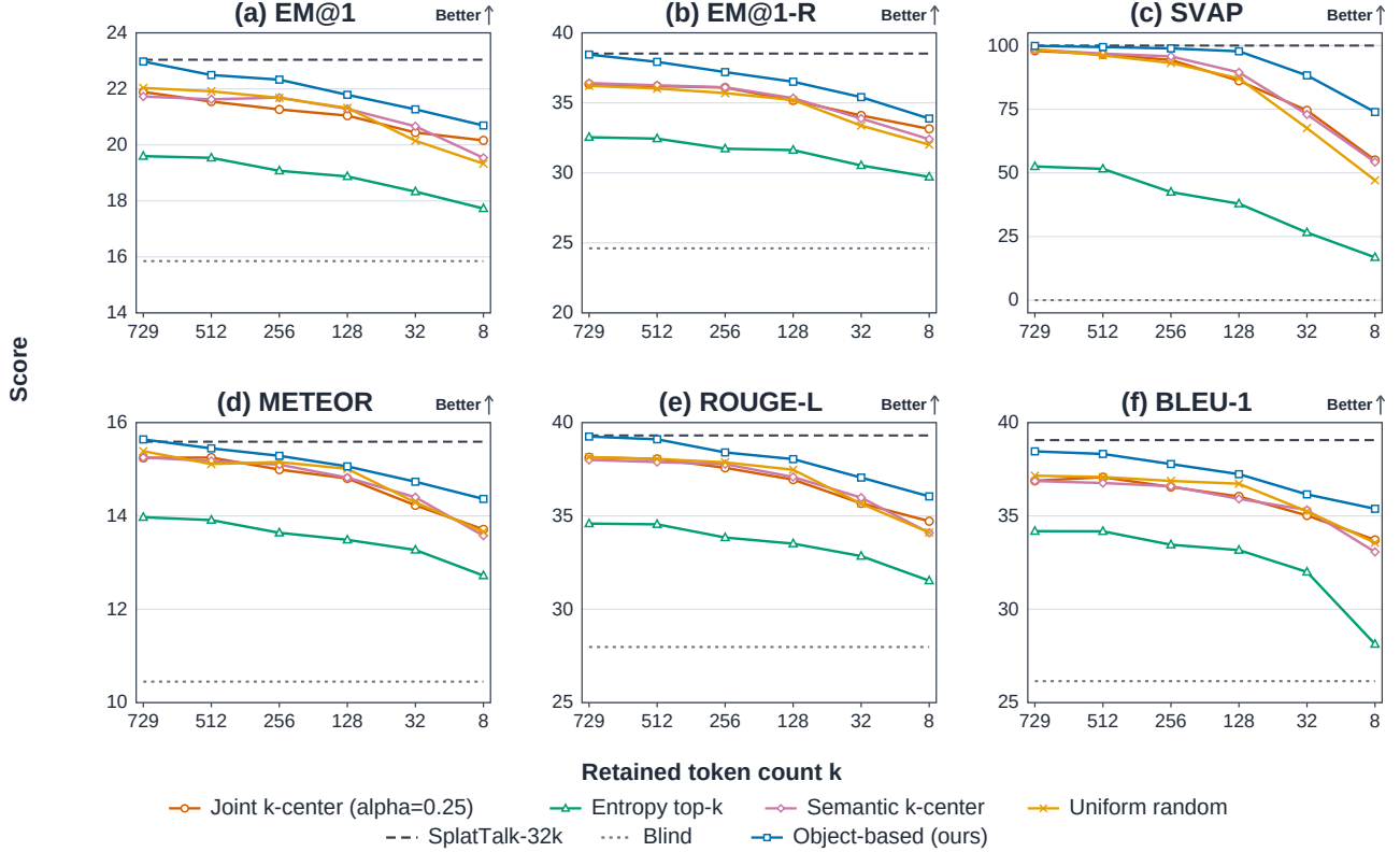
Figure 3. Performance on ScanQA when sparsifying from 729 down to 8 Gaussian embeddings, with the object-based selection offering the best results, maintaining performance down to 256 tokens. SplatTalk-32k denotes the original 32,076-token inference budget; Blind uses no visual tokens.
