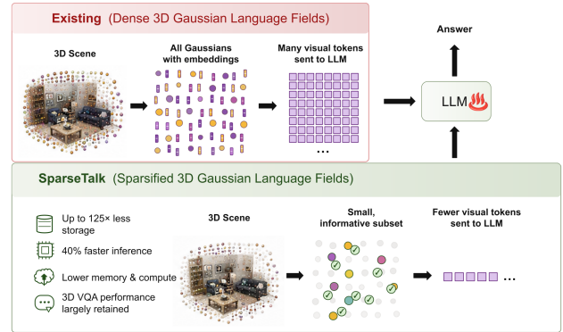
Figure 1. By using object-based sparsification, we reduce the number of semantic embeddings from tens of thousands to a few hundred, leading to faster inference and less memory usage, while retaining most of the VQA performance across the ScanQA and MV-ScanQA datasets.
