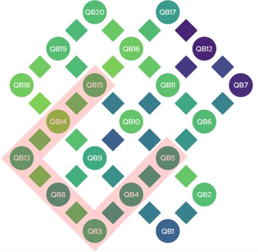
FIG. 5. Layout of the IQM Garnet QPU. The color map indicates single and two-qubit gate errors (darker=higher error, lighter=lower error). We highlight the optimal way to choose a qubit patch to implement a Hamiltonian evolution feature map with nearest-neighbour interactions. The specific patch needs to be adjusted depending on re-calibration of the QPU.
