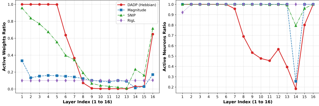
(a) Layer-Wise Sparsity Profile (90% Sparsity)
