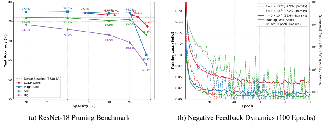
Figure 1: (a) Test accuracy versus sparsity for ResNet-18 on CIFAR-10. DADP maintains high accuracy up to 99.23% global sparsity. (b) Self-regulating negative feedback dynamics across three pruning thresholds ( \tau \in \{1e-6, 1e-5, 5e-5\} ) on MLP (MNIST, 100 epochs), illustrating training loss stabilization alongside decaying parameter pruning rates.
