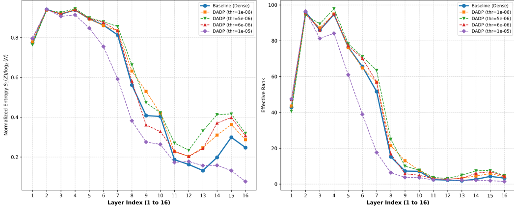
(b) Information-Theoretic Representation Quality (Matrix Entropy & Effective Rank)
