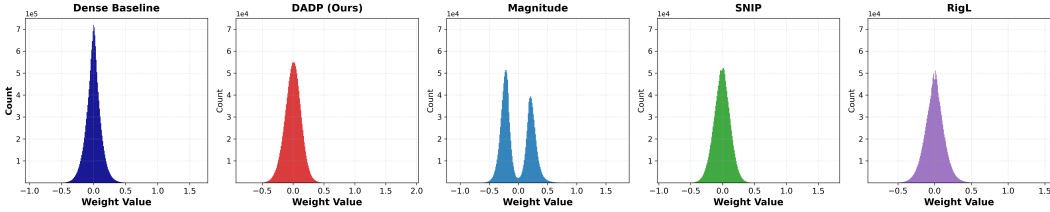
(c) Global Active Weight Value Distributions across Pruning Methods
