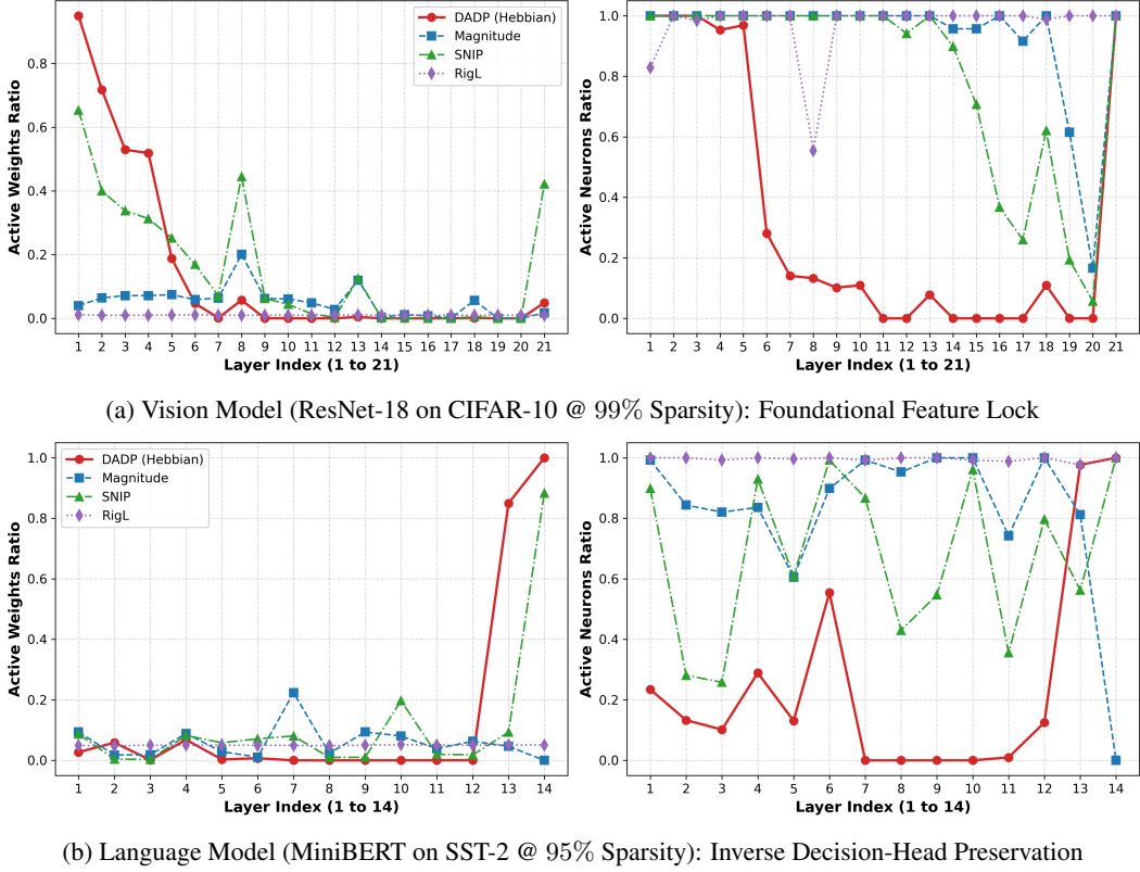
Figure 2: Layer-wise sparsity allocation across diverse architectural paradigms. Layer indices on the x-axis (1, 2, 3, ..., L ) correspond to sequential layer depths from input to output (full layer name mapping listed in Appendix Table 13). (a) Vision models (ResNet-18) preserve early visual feature extractors (0% sparsity) while compressing deep representations. (b) Sequence & Language models (MiniBERT) exhibit inverse allocation, heavily pruning early token projections while preserving dense capacity in deep attention decision heads. VGG-16 layer-wise sparsity profile is provided in Appendix E.
