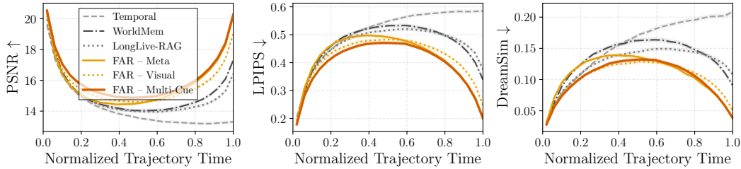
Figure 3: LoopNav rollout quality. We report frame-wise PSNR \uparrow , LPIPS \downarrow , and DreamSim \downarrow between generated and ground-truth return trajectories as a function of normalized trajectory time. Curves show the mean across trajectories, with shaded regions indicating 95% bootstrap confidence intervals. Errors are highest near the middle of the return phase, where relevant observations are typically farthest in time and memory is most sparse.
