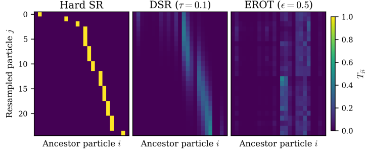
Figure 1: Transportation maps for systematic resampling (left), DSR (middle), and EROT (right), for a sequential important resampling PF of the Lorenz-63 system. The transportation maps are calculated at step 150 using N = 25 particles, and DSR and EROT uses training relaxation parameters.
