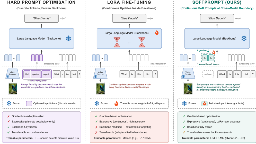
Figure 2: SOFTPROMPT combines the strengths of the two dominant adaptation approaches. Hard prompt optimisation (left) keeps the backbone frozen but searches a discrete vocabulary, which limits expressiveness on specialised domains and precludes gradient-based optimisation. LORA fine-tuning (centre) enables gradient-based adaptation and high accuracy, but modifies millions of backbone weights and risks catastrophic forgetting. SOFTPROMPT (right) optimises L continuous tokens at the cross-modal boundary of the multimodal sequence, reaching LORA-level accuracy while keeping the backbone fully frozen and training only L \times d parameters (8,192 at L=2 ; L is sized per domain, §5.2). Like hard prompts and unlike LORA, the learnt tokens transfer across models (§6.3) and can be verbalised into editable text (§6.2).
