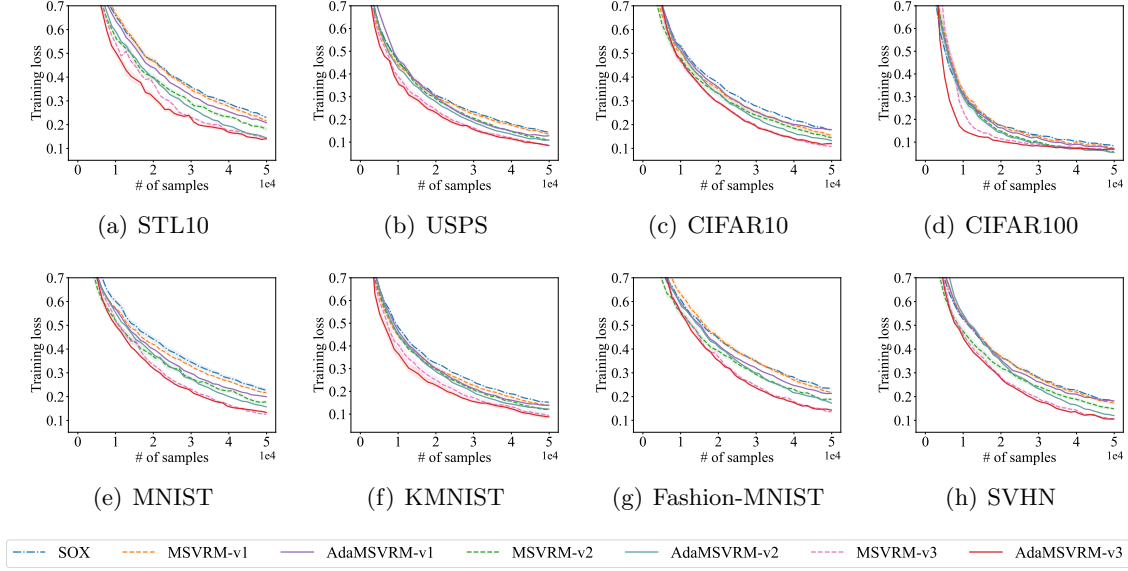
Figure 1: Training loss versus the number of samples for Multi-task AUC Optimization.
