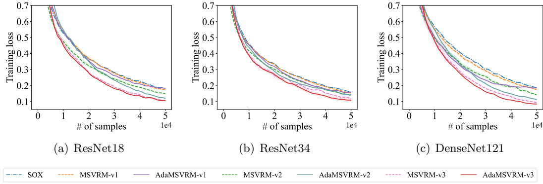
Figure 3: Results with different network architectures.
