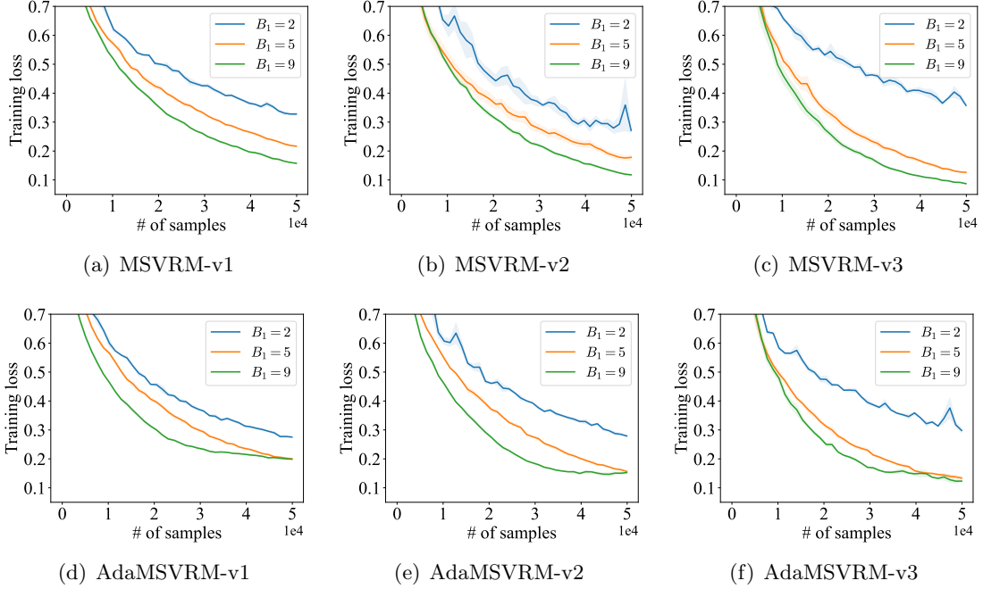
Figure 4: Results with varying outer batch size B_1 .
