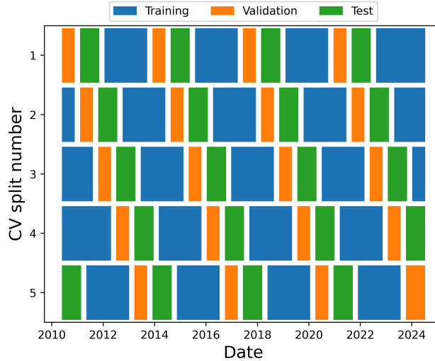
Figure 5. Cross-validation data splits of our dataset. Training and evaluation data is distributed over the solar cycle and 90 days are discarded between chunks to avoid data leakage.
