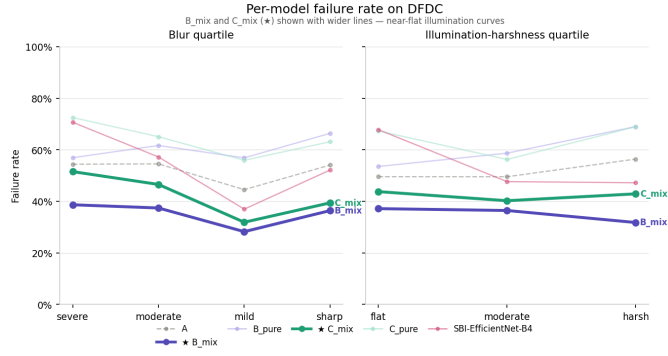
Fig. 3. Per-model failure rate on DFDC by blur quartile (left) and illumination-harshness bin (right). B_{\text{mix}} and C_{\text{mix}} —the T-SBI contrast—are near-flat on the illumination axis, with no preferential reduction on the harsh bin.
