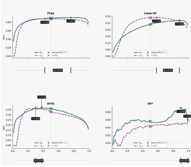
Fig. 2. MCC versus decision threshold for B_{\text{mix}} and C_{\text{mix}} , per dataset. Stars mark each model’s argmax; crosses mark threshold 0.5. The T-SBI variant’s optimum sits \approx 0.30 – 0.34 lower on FF++ and Celeb-DF, which is what makes threshold-0.5 comparisons misleading.
