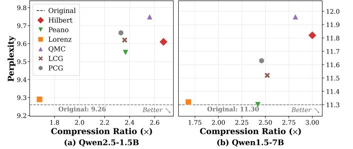
Fig. 5. Compression-PPL trade-offs on Qwen2.5-1.5B and Qwen1.5-7B. Dashed lines denote the PPL of the corresponding uncompressed models. Higher compression ratios and lower perplexity indicate better trade-offs.
