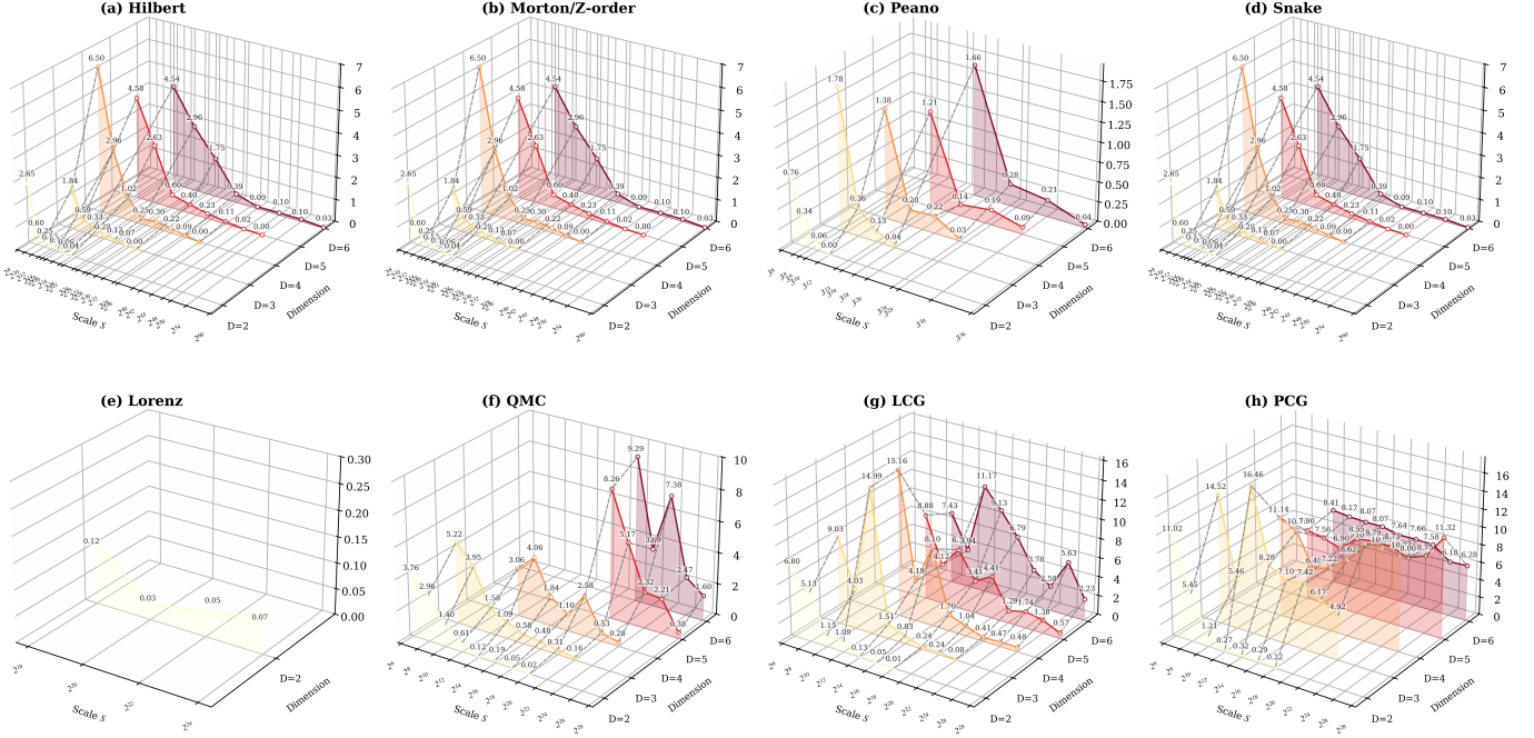
Fig. 4. Top-1 accuracy-drop landscapes of the eight evaluated methods on ResNet-18. The vertical axis reports the Top-1 accuracy drop relative to the original model in percentage points. Lower values indicate better accuracy preservation.
