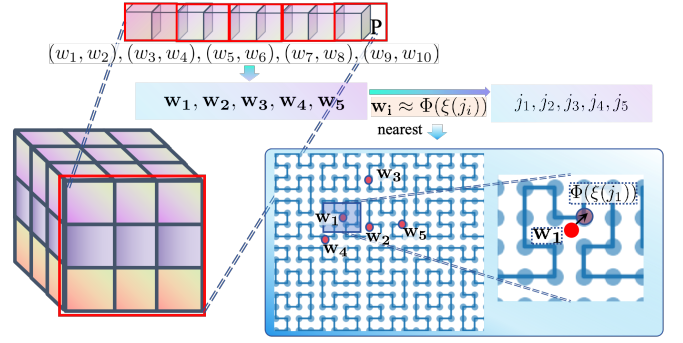
Fig. 2. An overview of the proposed DS-based compression framework. The parameter tensor is flattened and partitioned into grouped weight vectors, which are mapped into a tensor-wise local domain. A dynamic system generates a finite trajectory of states, and each grouped vector is assigned to its nearest state and the associated index. The model is compressed by storing the resulting index instead of the original floating-point vectors, while the states are recovered from the index for decompression.
