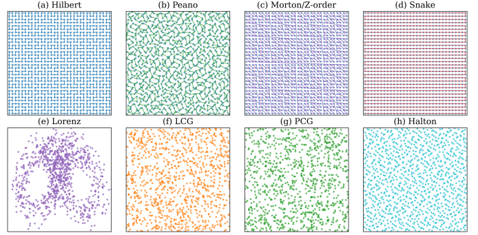
Fig. 1. Representative geometries generated by eight evaluated mapping families. Hilbert, Peano, Morton/Z-order, and Snake produce structured lattice traversals with different locality characteristics and traversal continuity. Lorenz generates a non-uniform attractor-induced distribution concentrated on a low-dimensional manifold. LCG and PCG produce deterministic pseudo-random point sets with different correlation structures, while Halton generates low-discrepancy coverage with reduced large-scale gaps. All methods are visualized after normalization to the same local domain.
