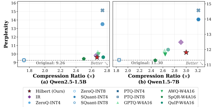
Fig. 6. Compression-perplexity trade-offs of weight-only compression methods on Qwen2.5-1.5B and Qwen1.5-7B. Higher CR and lower PPL indicate better trade-offs.
