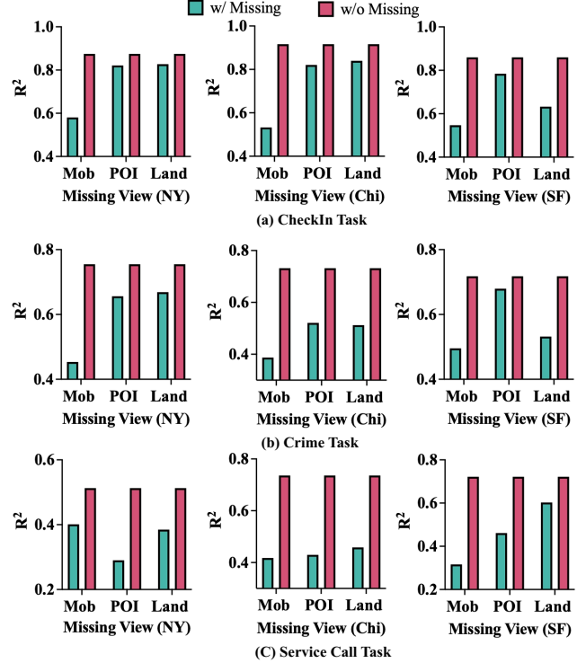
Fig. 6. Effects of missing views.
