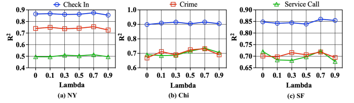
Fig. 4. Effects of Lambda ( \lambda ).
