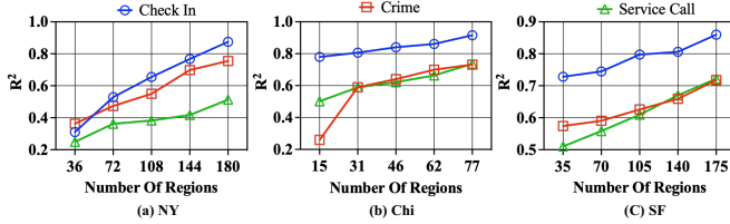
Fig. 5. Scalability Analysis with respect to the Number of Regions.
