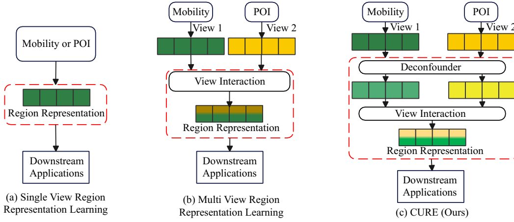
Fig. 1. Comparison of region representation learning paradigms. (a) Single-view region representation learning constructs embeddings from one urban data source, which limits its ability to capture heterogeneous urban semantics. (b) Conventional multi-view region representation learning integrates multiple views through general cross-view interaction, but may directly propagate correlation-induced shared signals. (c) CURE explicitly models potential latent confounding factors and performs confounder-aware view interaction before fusion, enabling the learned region representations to emphasize stable and task-relevant view-specific information for downstream urban analytics.
