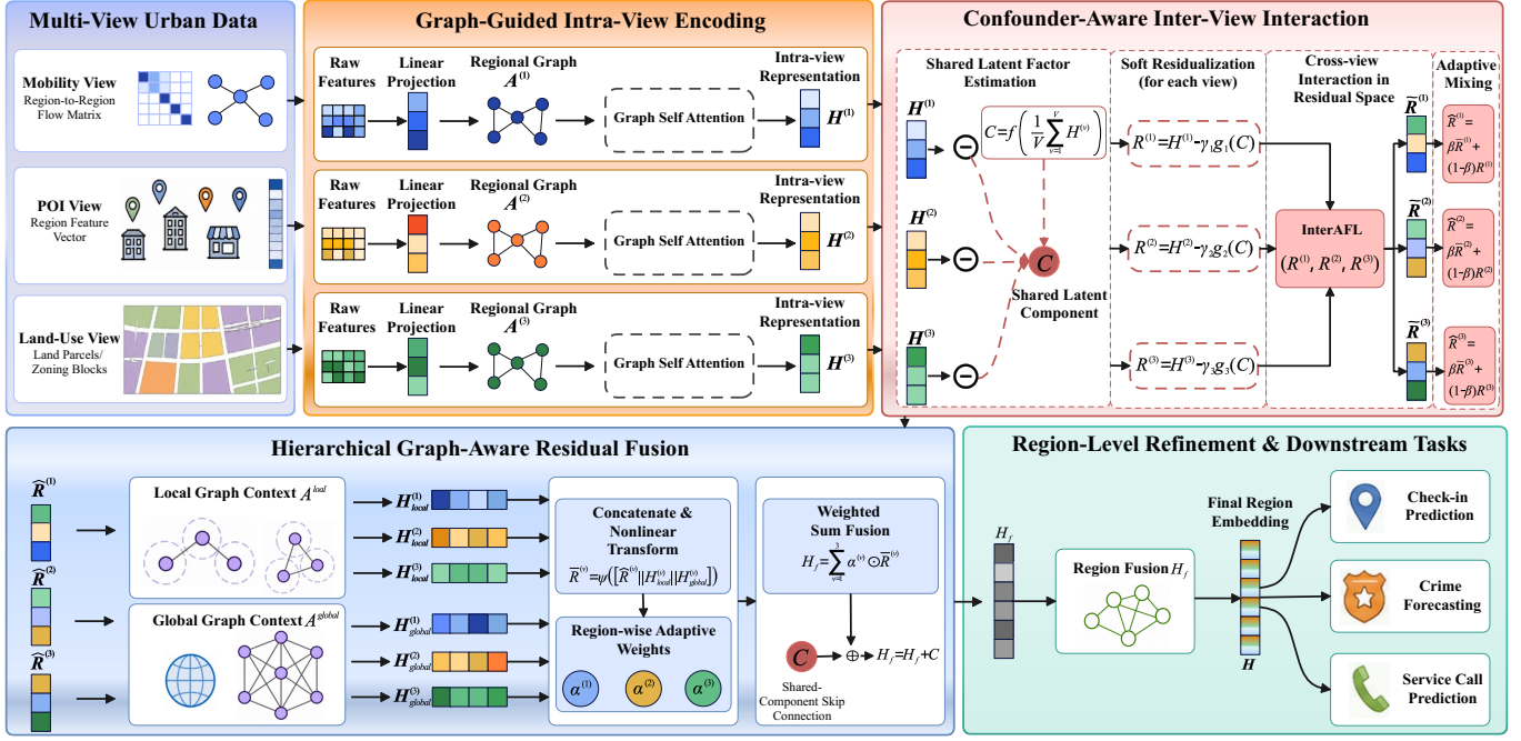
Fig. 2. Overview of CURE. CURE encodes mobility, POI, and land-use views with graph-guided intra-view encoders, estimates a shared latent component and reduces its projected influence before cross-view interaction, and adaptively fuses residual view representations under local and global graph contexts. The resulting region embeddings are used for downstream tasks such as check-in prediction, crime forecasting, and service call prediction.
