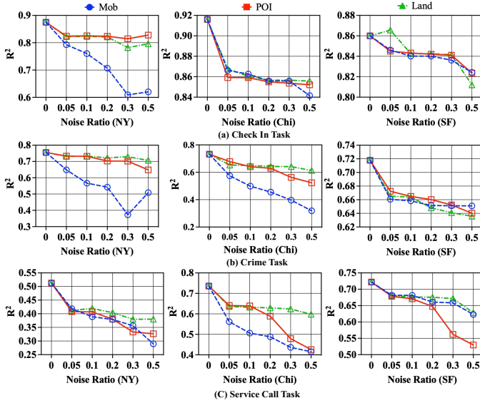
Fig. 7. Effects of feature noise.
