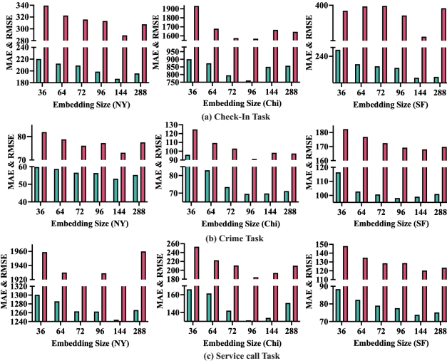
Fig. 3. Effects of Embedding Size.
