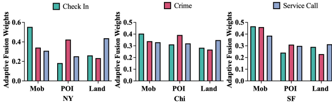
Fig. 8. Adaptive Fusion Weights Analysis.
