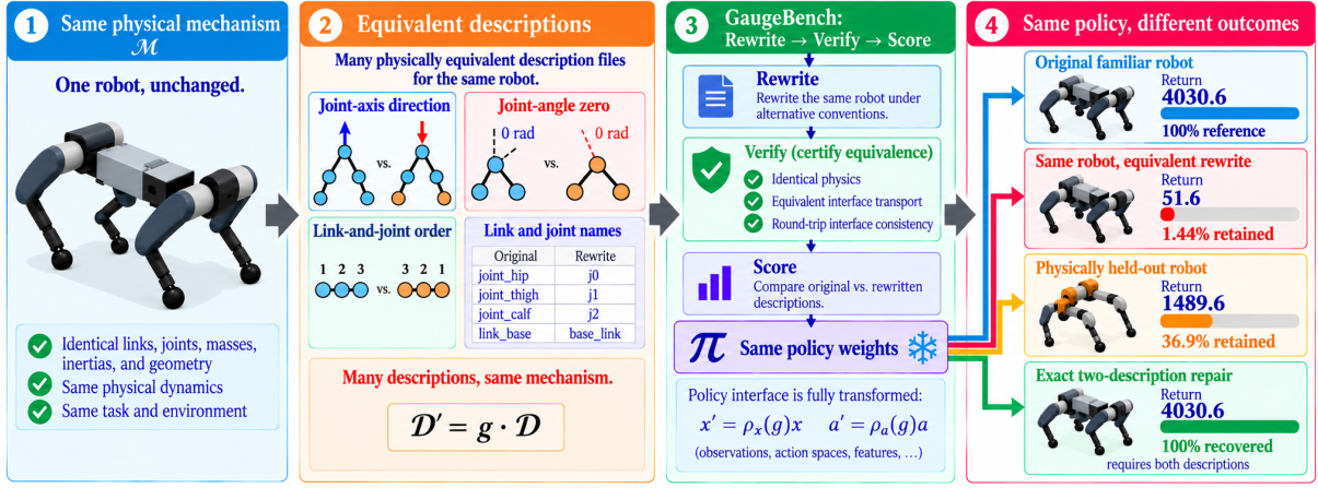
Fig. 1. One mechanism, many descriptions, and the evaluation axis that exposes them. A description records a mechanism together with arbitrary conventions: joint-axis directions \sigma_j , joint-angle zeros q_{0,j} , link-and-joint order p , and part names. GaugeBench rewrites a robot under a different choice of them, certifies physical and interface equivalence, and only then scores the same weights. MetaMorph keeps roughly a third of its return on a physically held-out robot but almost nothing on an equivalent rewrite of a robot it trained on.
