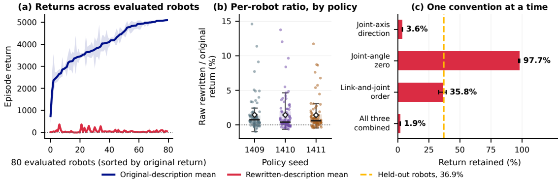
Fig. 3. The collapse is uniform across robots and policies, and one convention alone reproduces it. (a) Per-robot return on the 80 evaluated robots, sorted by original performance, with bands spanning the three policies. Rewritten return stays near zero across the entire range, so the mean is not carried by a few fragile robots. (b) Per-robot raw ratio of rewritten to original return, one column per trained policy. All 240 robot-policy pairs fall below 15 percent, and the axis is not truncated. (c) Do-nothing-adjusted return retained per convention, against the held-out reference. Joint-axis direction alone reaches the floor the combined rewrite reaches, while the joint-angle zero is nearly harmless. Error bars are the between-policy standard deviation, and these effects are not additive.
