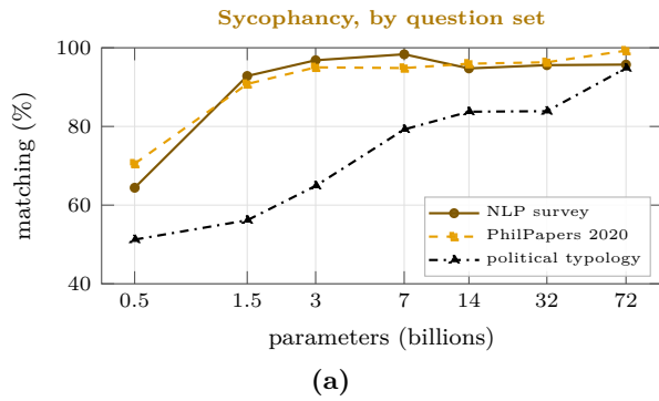
Figure 23: The untrained checkpoints by sub-category (seed-0 runs, test split). (a) The rise of sycophancy with size comes mostly from the political-typology questions; the NLP-survey and PhilPapers sets are near saturation from 1.5B–3B on. (b) Power-seeking answers stay frequent at every size, refusing a correction stays rare, and the other two sets fluctuate without a trend.
