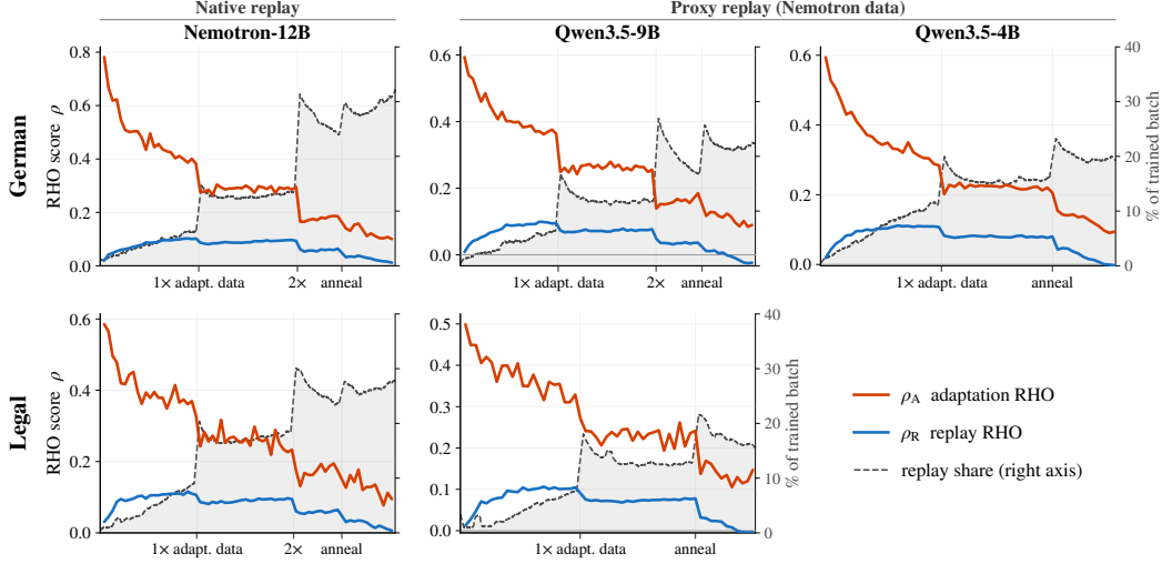
Figure 8: RHO-score dynamics across model-domain settings. Mean adaptation RHO score \rho_A and replay RHO score \rho_R over training, together with the resulting replay share. Across settings, adaptation scores decrease as the model learns the adaptation distribution, while replay scores initially increase as forgetting accumulates. The resulting competition between both signals dynamically adjusts the amount of replay throughout training. Vertical changes in replay share coincide with transitions between data passes and the learning-rate annealing phase.
