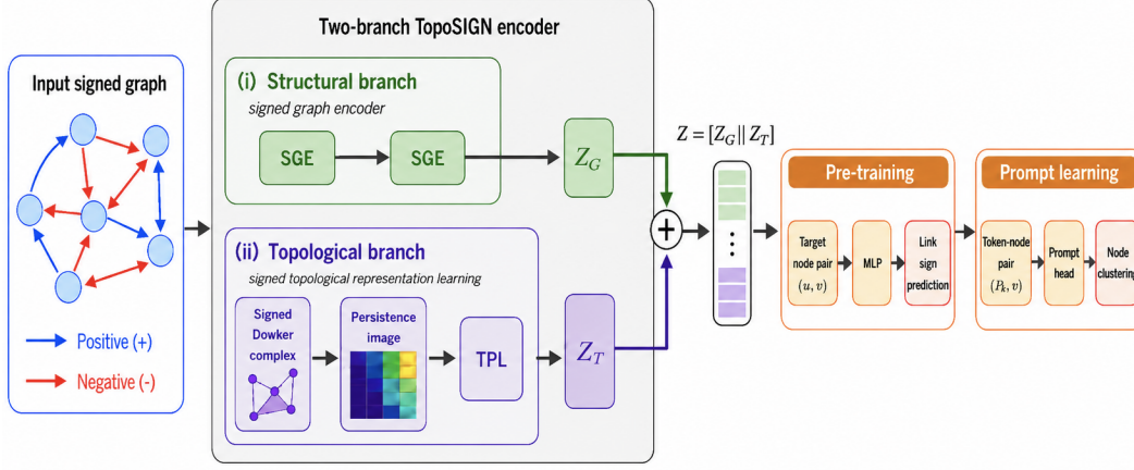
Figure 1: Overview of the TopoSIGN pre-training and prompting framework. Given an input signed (possibly also directed) graph with node attributes, TopoSIGN learns transferable representations through two complementary pathways (with the gray box). The first branch (i) applies signed graph encoder (SGE) layers to capture signed, directional, and local structural information. In parallel, the second branch (ii) constructs a Dowker complex to encode higher-order relational structures, which are transformed into compact topological embeddings via the topological representation learning (TPL) module using a projection layer. The structural and topological representations are fused to form joint node embeddings. Pre-training is performed using a pairwise prediction objective on both node-node and token-node pairs with a shared MLP and pretext loss, enabling topology-aware and prompt-compatible representations for downstream tasks.
