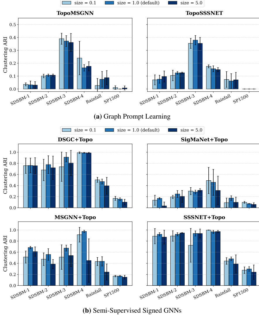
Figure 3: Downstream node clustering ARI sensitivity comparison across persistence image discretization resolutions ( \text{pixel\_size} \in \{0.1, 1.0, 5.0\} ) over diverse datasets. Bars from lighter to darker shades denote \text{pixel\_size} = 0.1, 1.0 (default), and 5.0 , respectively.
