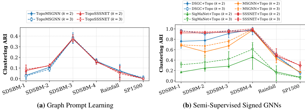
Figure 2: Downstream node clustering ARI sensitivity comparison across ego-network extraction radii ( k = 2 vs. k = 3 ) over diverse datasets. Solid lines represent k = 2 and dashed lines represent k = 3 .
