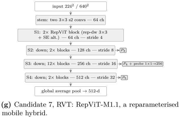
Figure 6: Eight candidate foundation models of the selection study. Every candidate exposes the same three feature maps (strides 8, 16 and 32, called P_3 to P_5 ) for the heads; the dashed 1x1 layer and the pooled endpoint exist only for pretraining. Candidate 3 became woma ; candidate 5, the runner-up, was fine-tuned on both models for comparison.
