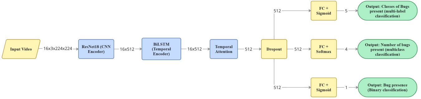
Fig. 3: ResNet-BiLSTM architecture.
