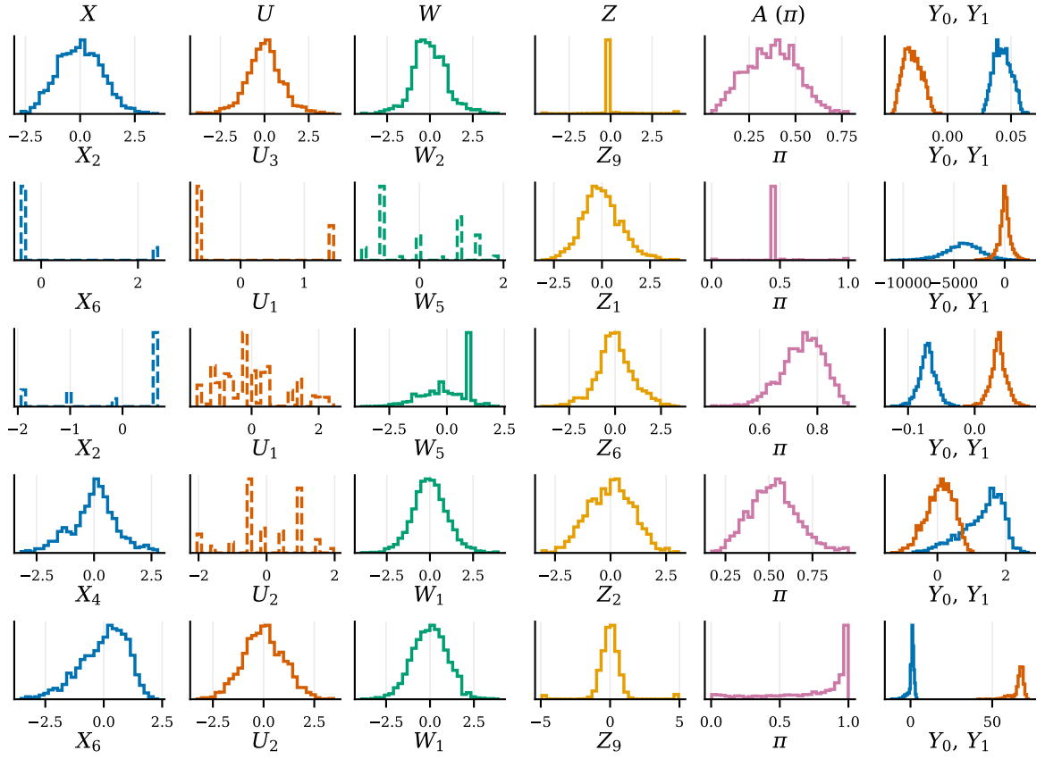
Figure B.10: Gallery of feature marginals: one column per block ( X , U , W , Z , the propensity \pi = P(A=1 \mid \cdot) for A , both potential outcomes for Y ), one row per randomly sampled dataset. Each panel is one feature column's histogram, solid for continuous columns and dashed for categorical ones; the Y column overlays Y_0 (blue) and Y_1 (red). Feature blocks share the standardised axis Corrupt leaves; \pi \in [0, 1] and Y keep their natural scale.
