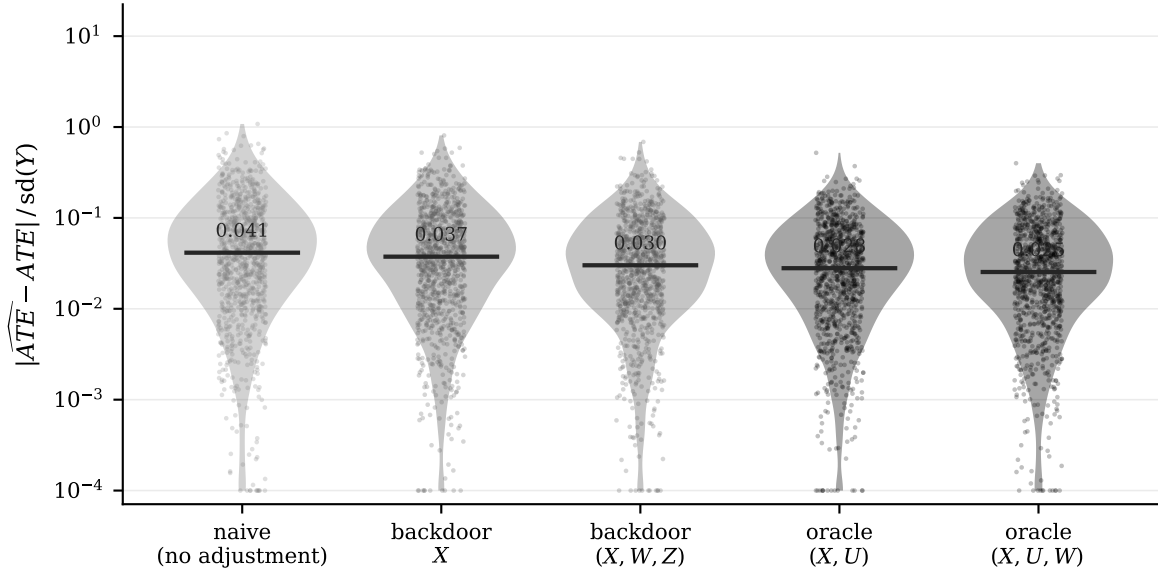
Figure B.15: Confounding-strength comparison (Table B.6) over 1024 datasets. Each violin shows normalised absolute ATE error |\widehat{ATE} - ATE|/sd(Y_{\text{obs}}) on a log axis, scored against \text{mean}(Y_1 - Y_0) : naive (no adjustment), backdoor X and (X, W, Z) (T-learners on measured covariates), and oracle (X, U) and (X, U, W) (T-learners also given the latent confounder).
