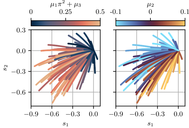
Figure 3: ADR test case: latent trajectories (AD-IC-LDNet). Test-set latent trajectories, translated to start from the origin, colored by \mu_1 \pi^2 + \mu_3 , which combines diffusion and reaction (left), and by the advection coefficient \mu_2 (right).
