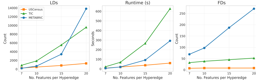
(a) Scalability of HLDT . With \tau_H = 0.2 , increasing the maximum hyperedge size recovers more LDs and FDs while increasing runtime.
