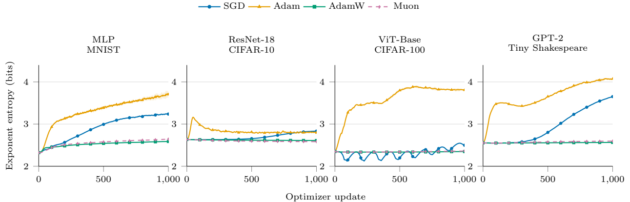
Figure 7: BF16 exponent entropy during early training. Lines and shaded bands show the mean \pm 1 sample standard deviation across three seeds. Models are trained from scratch on MNIST (LeCun et al., 1998), CIFAR-10 (Krizhevsky, 2009), CIFAR-100 (Krizhevsky, 2009), and Tiny Shakespeare (Karpathy, 2015), respectively, with matched initialization and minibatches across optimizers. Training uses random initialization and matched minibatch order (seeds 17, 29, 43). Effective batches are 128 (images) and 32 (GPT-2, 128 tokens), with ViT/GPT-2 microbatches 8/4. SGD rates are 0.05 (images)/0.1 (GPT-2), Adam/AdamW/Muon rates are 10^{-3} (MLP/ResNet-18)/ 3 \times 10^{-4} (ViT/GPT-2). We use a 50-update linear warm-up, norm-1 clipping, and a weight decay of 0.01 for matrix/convolution weights, zero otherwise. Images use official train/test splits, fixed channel standardization, no augmentation, and 224 \times 224 bilinear ViT resizing, Tiny Shakespeare uses GPT-2 BPE and a contiguous 90%/10% train/hold-out split. Full optimizer parameters, preprocessing constants, architecture adjustments, and evaluation settings are specified in the anonymized repository.
