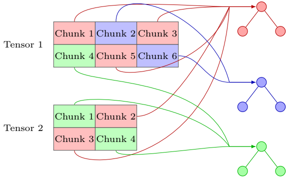
Figure 4: Sharing codebook example.
