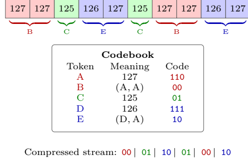
Figure 5: Packed exponents example.
