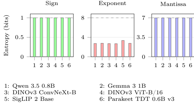
Figure 1: Empirical entropy by floating-point field in BF16.
