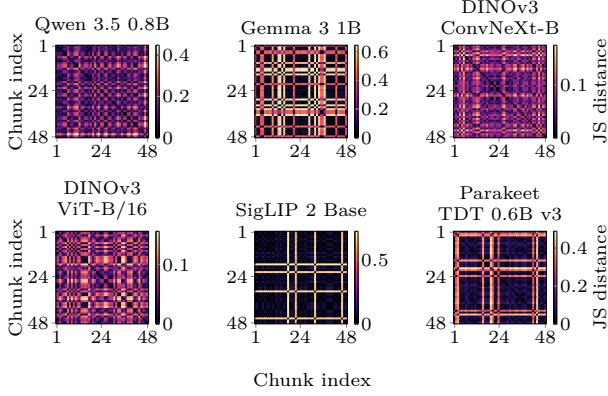
Figure 2: Jensen–Shannon distances between exponent histograms of 48 sampled chunks per model.
