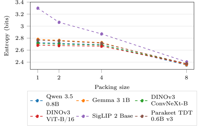
Figure 3: Local exponent redundancy entropy.
