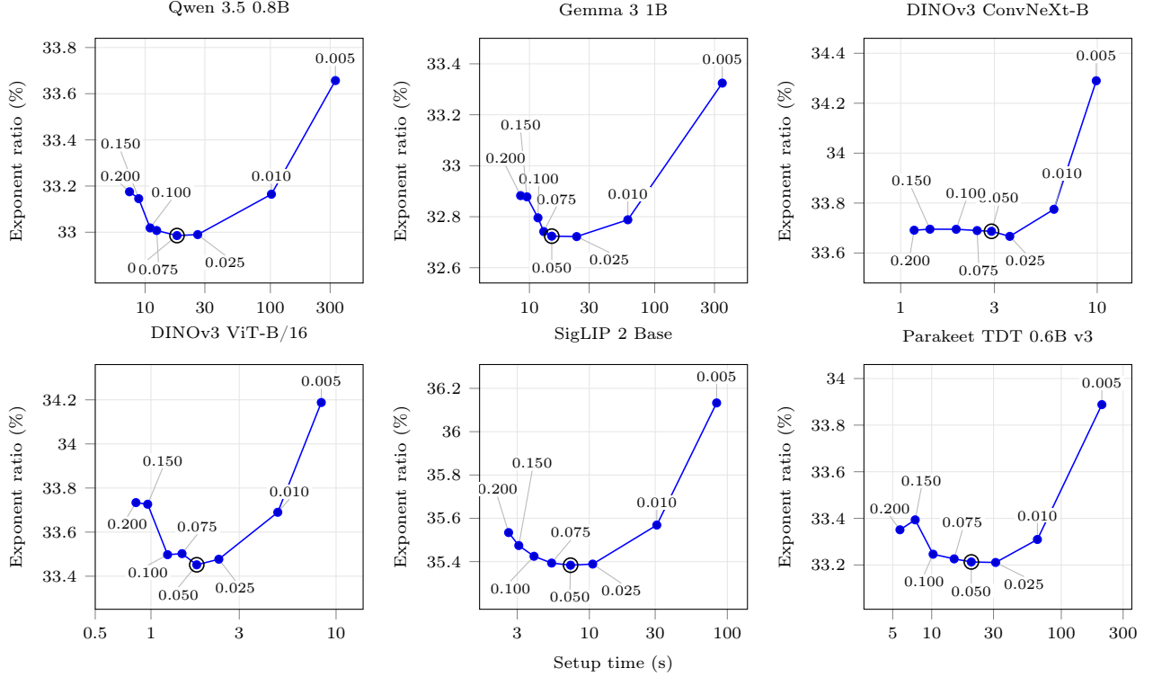
Figure 8: Own-setup JS-threshold sweep. Circles mark the default \tau = 0.05 .
