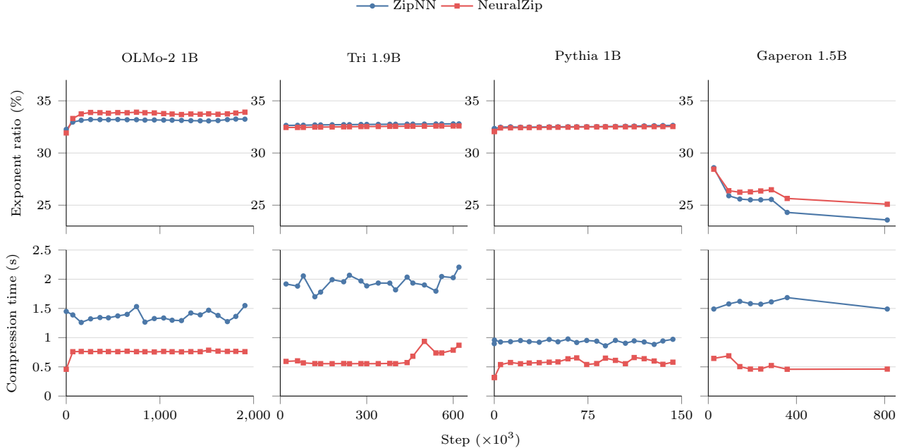
Figure 6: Compression across training checkpoints. We keep each family’s earliest setup frozen.
