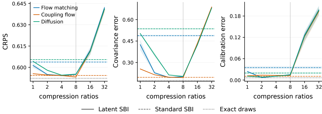
Figure 5: Compression ratio study for the Correlated Gaussian example. Given latent dimension d , the latent compression ratios are 64/d . For each ratio, we evaluate the continuous ranked probability score (CRPS; left ), covariance error ( middle ), and calibration error ( right ) against their standard SBI baselines for three inference networks: flow matching, normalizing flow, and diffusion model.
