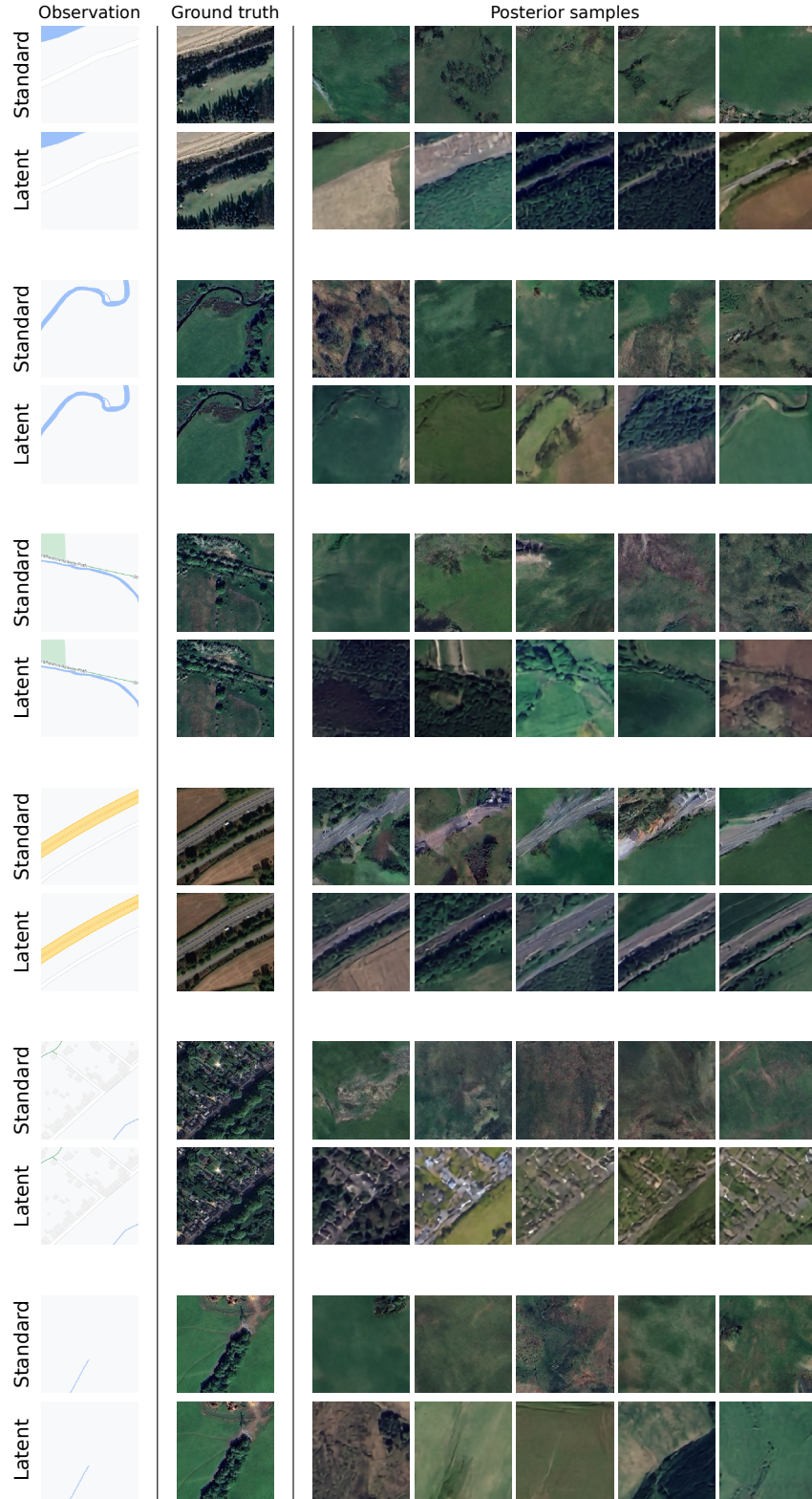
Figure 10: Random conditions for map to satellite. Posterior samples for six map-to-satellite test conditions drawn at random, not selected, as in Figure 4.
