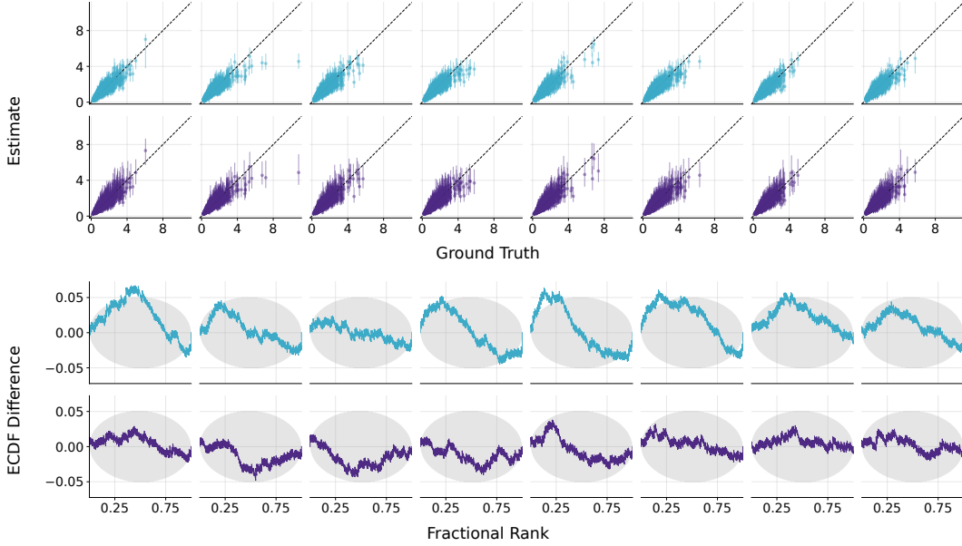
Figure 2: Recovery and calibration on the correlated Gaussian. Parameter recovery ( top ) and calibration ECDFs (Säilynoja et al., 2022) ( bottom ) of standard SBI ( blue , first row of each) and latent SBI ( purple , second row of each) for the correlated Gaussian with flow matching, one column per block variance \sigma_1^2, \dots, \sigma_8^2 . Latent SBI achieves notably better calibration than standard SBI, as no ECDF leaves the simultaneous confidence bands. A comparison against the exact posterior is in Appendix G.
