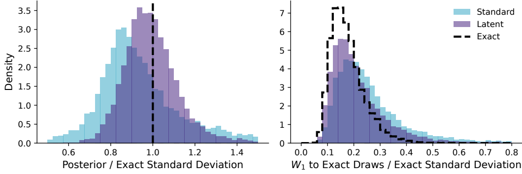
Figure 6: Comparison against the exact posterior on the correlated Gaussian. With flow matching, on the k = 8 block variances (1,000 test conditions, 100 draws each). Left: posterior standard deviation relative to the exact one. Latent widths scatter evenly around the exact width, while standard widths are too narrow for most conditions and far too wide for some. Right: Wasserstein-1 distance ( W_1 ) to exact draws, relative to the exact standard deviation; the dashed outline shows the sampling noise of the exact posterior itself.
