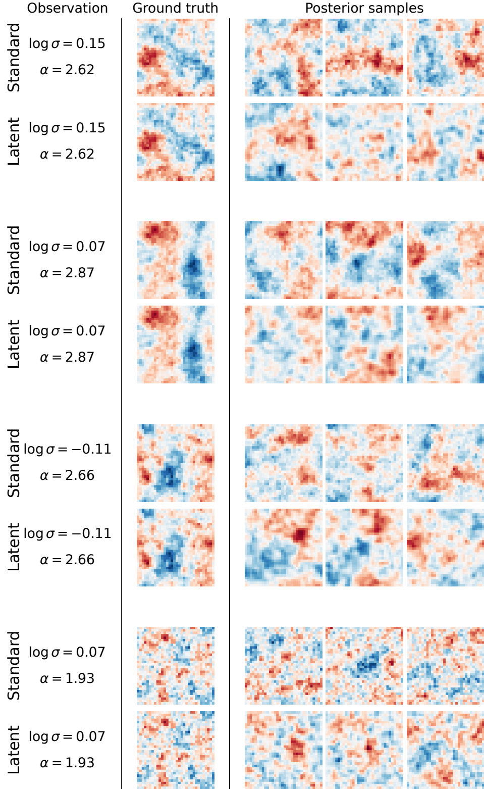
Figure 8: Random conditions for the Gaussian random fields. Posterior samples for four random-field test conditions drawn at random, not selected, as in Figure 3b. Colors share one symmetric scale per condition.
