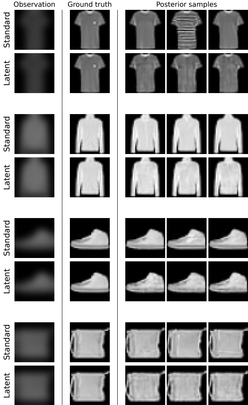
Figure 7: Random conditions for Fashion-MNIST deblurring. Posterior samples for four Fashion-MNIST test conditions drawn at random, not selected, with flow matching.
