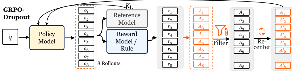
Figure 1: GRPODropout procedure. Filter removes only selected positive-advantage rollouts; Re-center applies probability-weighted advantage recentering. Other GRPO updates are unchanged.
