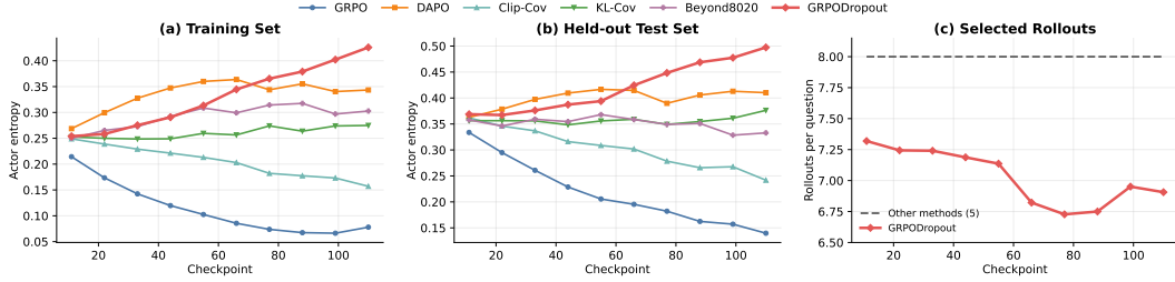
Figure 2: Qwen3-4B actor entropy and rollout usage across checkpoints. (a–b) Token-mean entropy on training DAPO-17K and held-out MMLU-Pro (MMLUP); (c) mean update rollouts per question in training batches, excluding all-zero-advantage groups. The other five methods use 8 rollouts at every recorded checkpoint (gray dashed line). Curves connect raw observations without smoothing.
