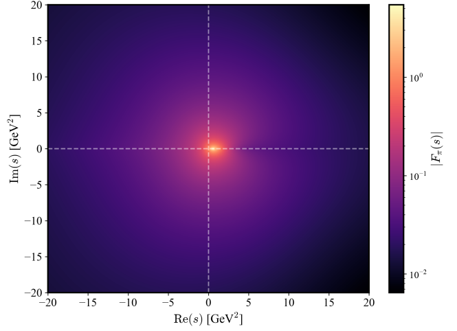
FIG. 4. Heat map of |F_\pi(s)| confirming that the predicted form factor contains no zeros in the interior of the \mathcal{S} plane.
