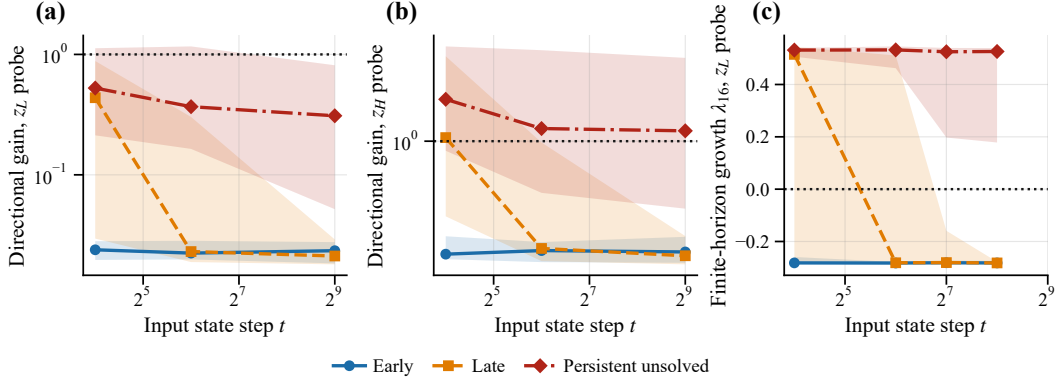
Figure 6: (a,b) Median one-step directional gain for probe directions supported on Z_L and Z_H , shown by group and input-state step. (c) Finite-horizon growth \lambda_{16} following a perturbation to Z_L . Shaded regions show interquartile ranges.
