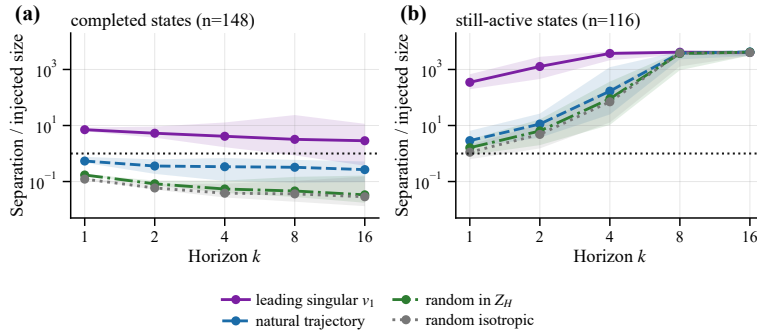
Figure 11: MLP response to norm-matched perturbations with initial size 10^{-4} of the state norm. Results are separated according to whether the unperturbed computation has already completed. Panel (a) pools the 100 fixed-step and 48 solve-aligned completed states (the text quotes fixed-step medians), and panel (b) shows the 116 still-active states. Shaded regions show interquartile ranges.
