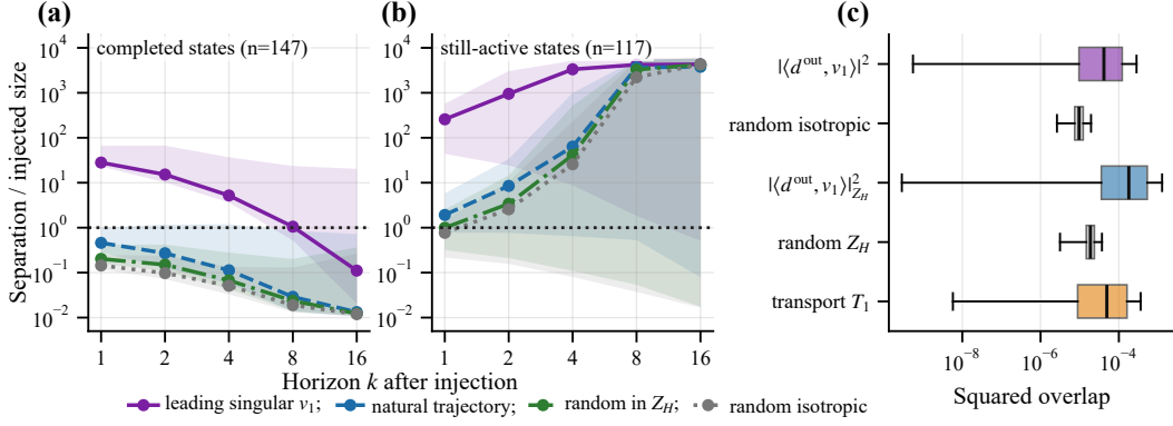
Figure 4: An expanding direction is present, but the trajectory is not orthogonal to it. Norm-matched perturbations ( 10^{-4} of the state norm) along four directions, followed for k further steps, at (a) states whose computation has completed and (b) states still computing. In (b) every direction, including a random one, reaches the scale of the state itself. These curves measure trajectory divergence. (c) Squared overlaps: the trajectory’s overlap with v_1 is tiny but distinctly above the isotropic baseline. The transport of the leading direction across one step is of the same order. The “random isotropic” is the overlap of v_1 with a random unit direction drawn uniformly from the full hidden-state space, and “random Z_H ” uses a random unit direction drawn from the Z_H subspace only.
