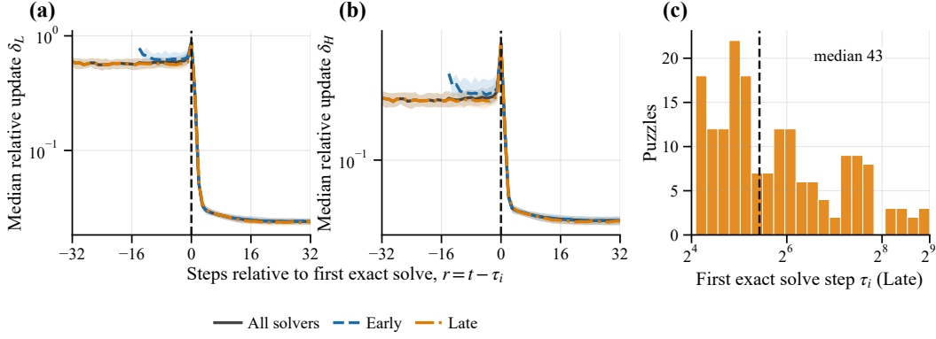
Figure 8: MLP solve-aligned dynamics. (a,b) Relative updates along the solve-aligned axis. (c) Distribution of first solve times for LATE solvers.
