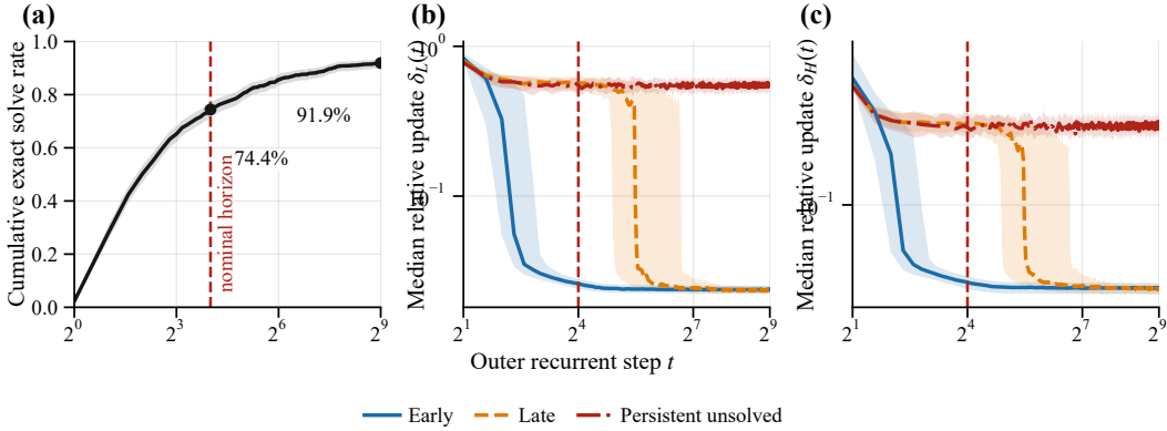
Figure 7: MLP extended recurrence. (a) Cumulative exact solve with Wilson bands. (b,c) Median relative latent update by completion group with interquartile bands.
