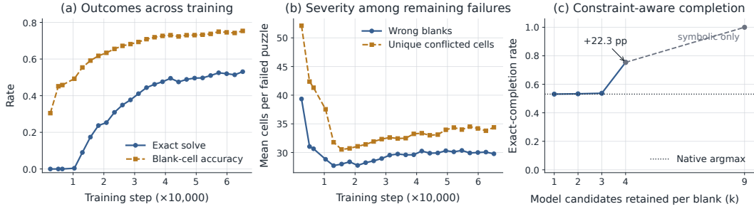
Figure 12: Attention-B training and decoder diagnostics. (a) Exact-solve and blank-cell accuracy across 25 correlated training snapshots. (b) Conflict severity. (c) Exact completion under model-guided Sudoku constraints; the dotted line is native argmax and k = 9 is a symbolic-only control.
