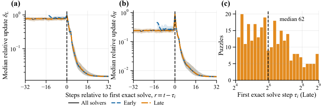
Figure 2: Settling is aligned to each puzzle’s own completion. (a,b) Median relative update on the solve-aligned axis r = t - \tau_i , with interquartile bands. Motion is roughly constant before completion, spikes at r = 0 , and then falls by more than an order of magnitude. The EARLY and LATE curves coincide once aligned, although their absolute solve times differ by an order of magnitude. (c) Distribution of \tau_i for LATE solvers.
