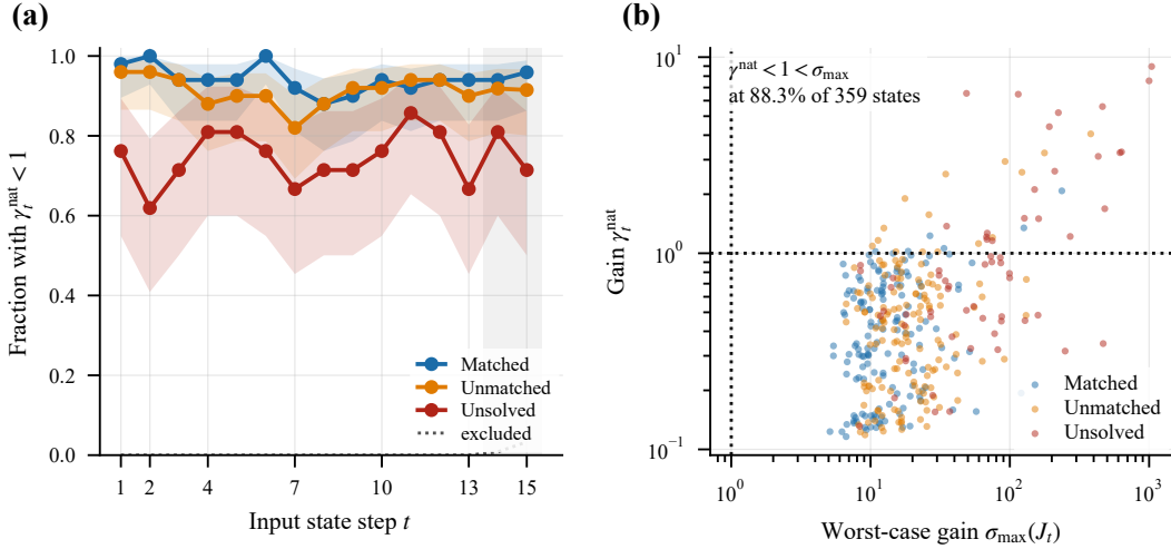
Figure 14: Directional contraction and worst-case expansion. (a) Fraction of valid directions with \gamma_t^{\text{nat}} < 1 , with Wilson bands. (b) States with both a valid directional gain and a singular-value estimate, at t = 2, 7, 15 . The inequalities \gamma_t^{\text{nat}} < 1 < \sigma_{\text{max}}(J_t) hold together at 317/359 states (88.3%).
