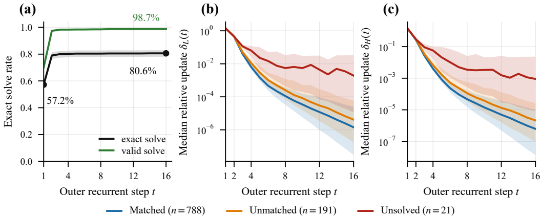
Figure 13: Maze-Hard outcomes and latent settling. (a) Cumulative exact solves from bfloat16 run, with Wilson bands. Figures (b,c) Median relative latent updates in float64. Shaded bands show interquartile ranges.
