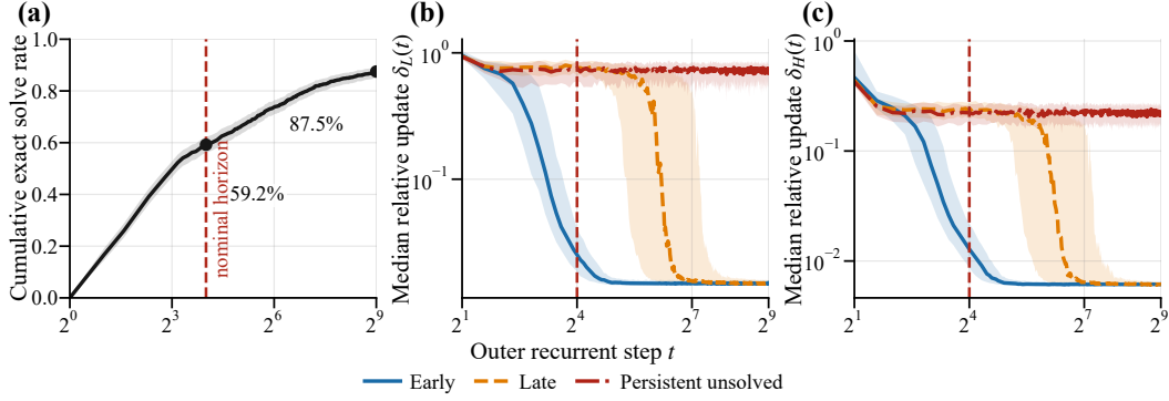
Figure 1: The nominal horizon truncates active computation. (a) Cumulative exact solve rate over 512 outer steps with Wilson bands; the dashed line is the nominal 16-step budget. (b,c) Median relative latent update with interquartile bands for the three completion groups. LATE solvers are as mobile as PERSISTENT ones at step 16 and settle only when they solve. PERSISTENT trajectories never settle.
