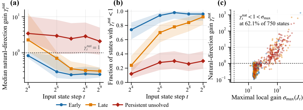
Figure 3: Stability is conditioned on the direction of travel. (a) Median natural-direction gain \gamma_t^{\text{nat}} by group and input-state step, with interquartile bands. The dotted line is \gamma_t^{\text{nat}} = 1 . (b) Fraction of states with \gamma_t^{\text{nat}} < 1 , with Wilson bands. (c) Every probed state: \gamma_t^{\text{nat}} against \sigma_{\text{max}}(J_t) . No state has \sigma_{\text{max}} < 1 , yet most completed states sit below \gamma_t^{\text{nat}} = 1 .
