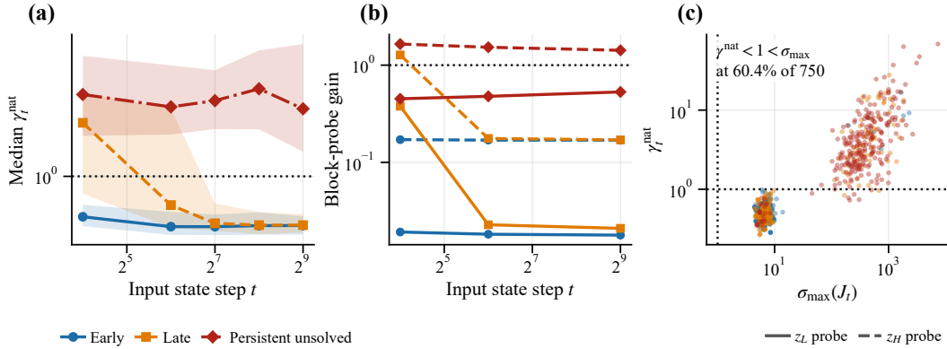
Figure 9: MLP local stability at fixed recurrent steps. (a) Median natural-direction gain by group. (b) Probe gains supported on Z_L (solid) and Z_H (dashed). (c) Natural-direction gain \gamma_t^{\text{nat}} versus \sigma_{\max}(J_t) for all probed states.
