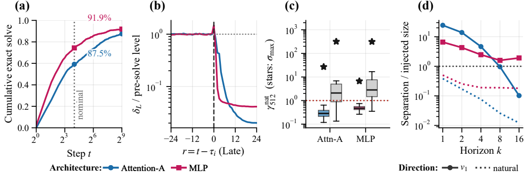
Figure 5: The completion geometry reproduces across architectures. Attention-A in blue, MLP in red. (a) Cumulative exact solve with extended recurrence, with the nominal horizon marked. (b) LATE-solver \delta_L on the solve-aligned axis, each model normalized by its own pre-solve level. (c) Natural-direction gain at step 512 for completed (colored) and PERSISTENT (grey) states, with the red line at \gamma^{\text{nat}} = 1 and stars marking median \sigma_{\text{max}} at the same states ( \sigma_{\text{max}} > 1 at every probed state in both models). (d) Norm-matched perturbations at completed fixed-step states along v_1 (solid markers) and along the natural direction (dotted). Both models expand v_1 and contract the natural direction, but only Attention-A absorbs the v_1 perturbation within 16 steps.
