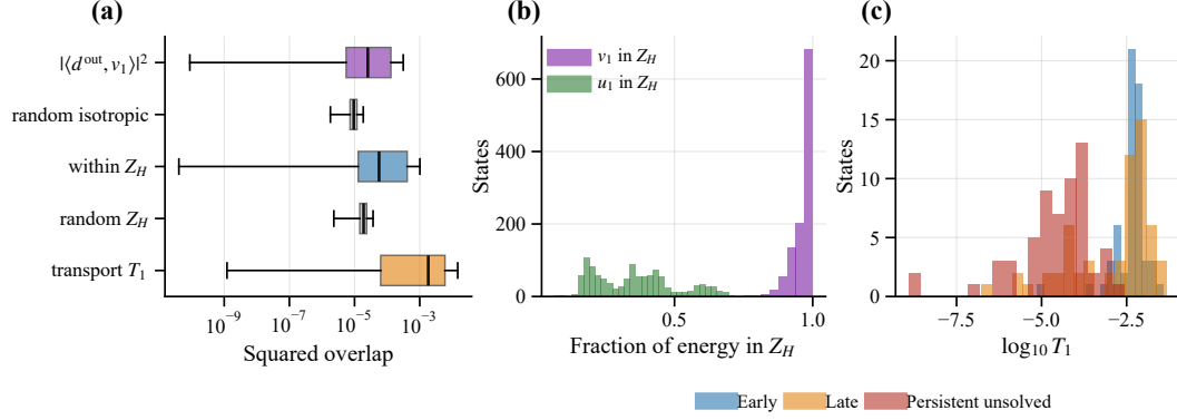
Figure 10: MLP leading singular-vector geometry. (a) Squared overlaps and one-step transport for the fixed-time states, together with random baselines. The “random isotropic” is the overlap of v_1 with a random unit direction drawn uniformly from the full hidden-state space, and “random Z_H ” uses a random unit direction drawn from the Z_H subspace only. Transport is evaluated on the 180-state subset. (b) Fraction of the leading right and left singular vectors supported on Z_L and Z_H . (c) Distribution of \log_{10} T_1 across completion groups.
