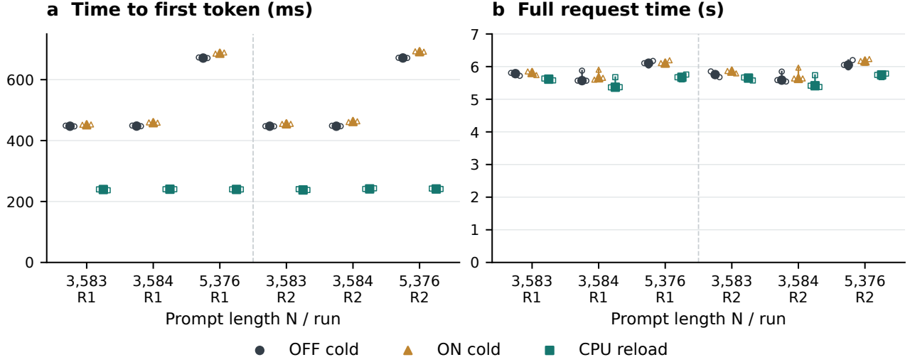
Figure 3: Serial latency measurements. Hollow points show three measured requests per run, length, and condition; filled markers show medians, and thin bars show observed min-max ranges, not confidence intervals. R1 runs OFF then ON; R2 reverses engine order. Both panels use the same 54 requests and zero-based axes. OFF is the modified no-connector control. The cold conditions have similar TTFT; total time includes the full 128-token generation.
