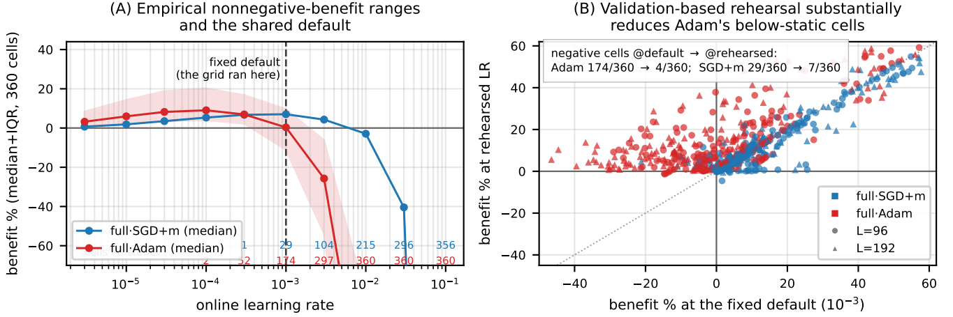
Fig. 3. Learning-rate sensitivity across all 360 cells. (A) Adaptation benefit by online learning rate, summarized by the median and interquartile range across cells; numbers along the bottom give the count of cells below the static baseline at each rate. The dashed line marks the shared default, 10^{-3} . (B) Per-cell benefit at the shared default ( x -axis) versus the validation-rehearsed rate ( y -axis); color denotes optimizer and marker shape denotes lookback length.
