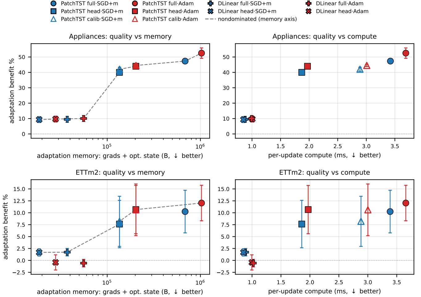
Fig. 4. Accuracy–resource characterization (C3) at validation-selected warmup and rehearsed learning rates (five seeds; mean \pm standard deviation). Adaptation benefit is plotted against adaptation-state memory (gradient buffers + optimizer state; left) and A100-measured per-update time (right) for Appliances (top) and ETTm2 (bottom). Color denotes optimizer (blue: SGD+m; red: Adam); marker shape denotes backbone and parameter subset (PatchTST: circle/square/triangle for full/head/calib; DLinear: plus/cross for full/head). Dashed links identify nondominated mean points on the memory axis; hollow calib markers overlay head markers because their adaptation-state memory differs only by the 2C calibration parameters.
