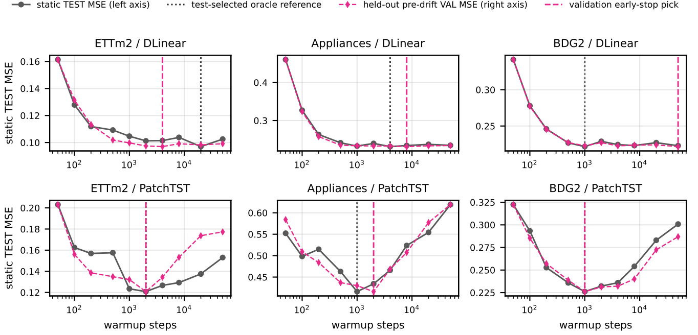
Fig. 2. Validation-only warmup selection on the study milestone grid and panel layout of Fig. 1 (three seeds; mean \pm standard deviation). Gray and magenta curves show static test MSE (left axis) and held-out pre-drift validation MSE (right axis), respectively. The magenta dashed and black dotted rules mark the validation early-stop and test-selected oracle warmups. The validation-MSE scale is suppressed because only its argmin is used for selection.
