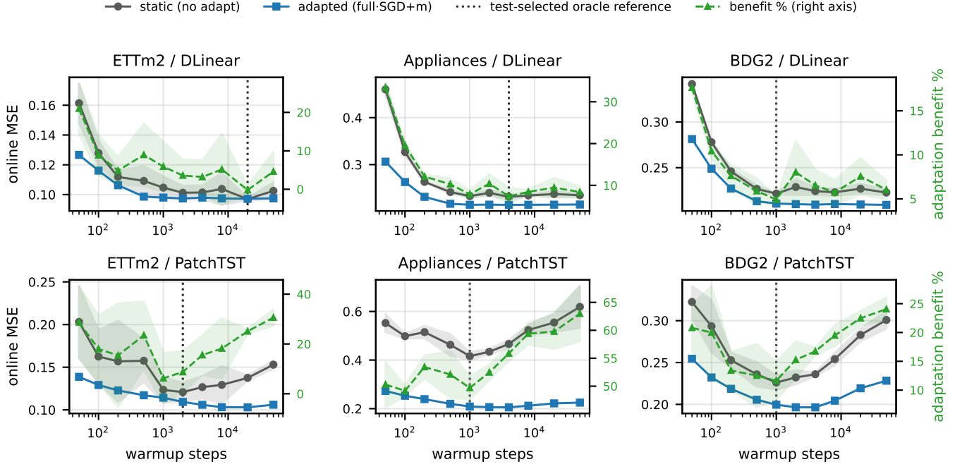
Fig. 1. Warmup sensitivity on the study milestone grid (three seeds; mean \pm standard deviation). In each dataset-backbone panel, gray and blue curves show the online test MSE of the static and full-SGD+m adapted models, respectively (left axis), and the green curve shows adaptation benefit (right axis). The black dotted rule marks the test-selected oracle warmup.
