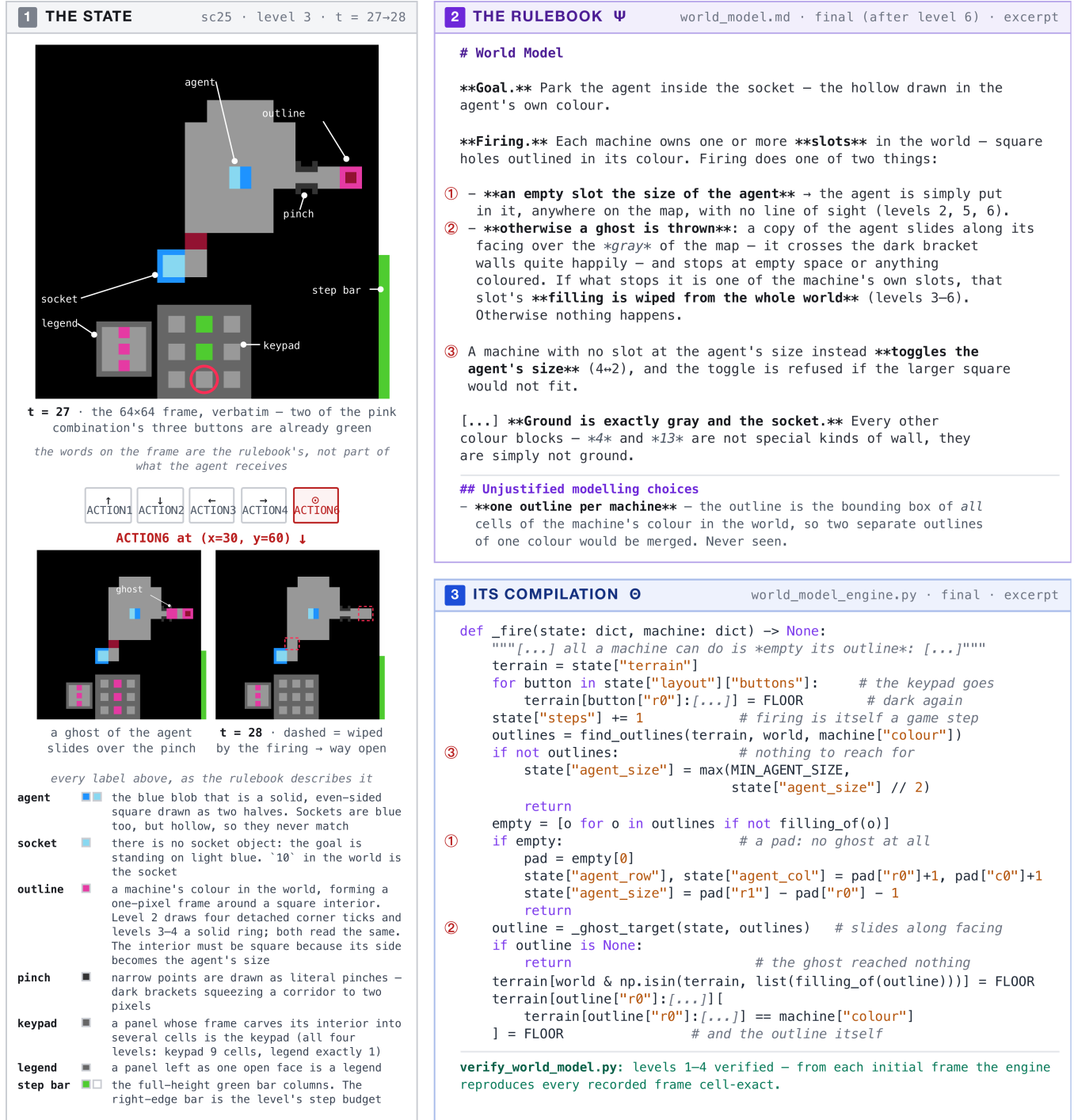
Figure 4: An ARC-AGI-3 realisation of a rulebook and its executable. Left: an observed transition from game sc25. Upper right: the final rulebook in world_model.md, whose names are also used to annotate the frame. Lower right: an excerpt from world_model_engine.py implementing the numbered rules. The executable is checked by cell-exact replay before it is used for planning.
