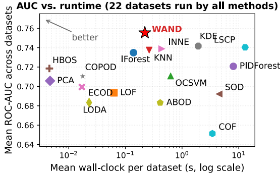
Fig. 9. Mean ROC-AUC vs. mean wall-clock per dataset (log x ), averaged over the 22 ADBench datasets completed by every method so all means cover the same tasks. WAND sits on the AUC–runtime Pareto frontier (top-left): no other method is both faster and more accurate on this shared subset. The subset necessarily excludes the largest datasets, on which the neighbour-based methods (LOF, kNN, ABOD, COF, SOD, LSCP, KDE, OCSVM) exceed the time budget, whereas WAND runs on all 47 (Table II).
