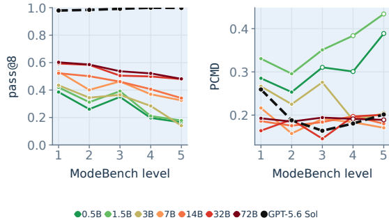
Figure 4: Correctness and solution-mode diversity vary across benchmark levels. Across increasingly difficult MODEBENCH levels, pass@8 generally declines, while PCMD follows different patterns across models.
