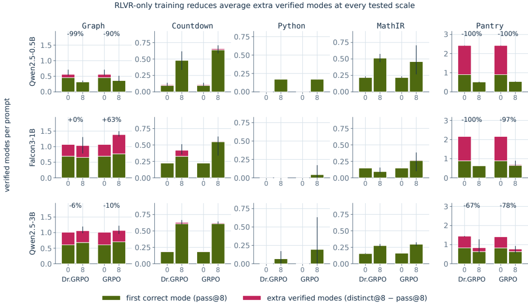
Figure 21: RLVR-only training reduces additional verified modes across scales. Bars decompose \text{distinct@8} into \text{pass@8} and additional verified modes before training and after eight passes for Dr.GRPO and GRPO across three model scales and five domains. Whiskers show ranges across five training seeds.
