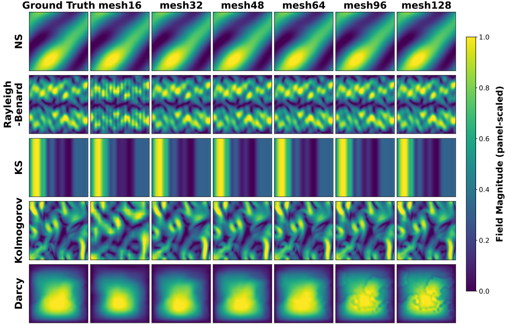
Figure 9: GA-AMNO predictions under cross-resolution evaluation. Columns show the ground truth and predictions at mesh resolutions 16, 32, 48, 64, 96, and 128; rows correspond to the five PDE benchmarks. The native training resolution is 64, and colors are independently scaled within each panel.
