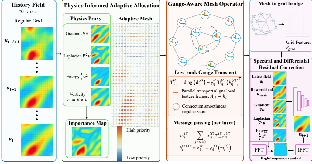
Figure 3: Overall architecture of GA-AMNO. Physics-informed indicators guide adaptive allocation, low-rank gauge transport aligns features before aggregation on the resulting mesh, and the reconstructed grid features are refined by spectral and differential residual corrections.
