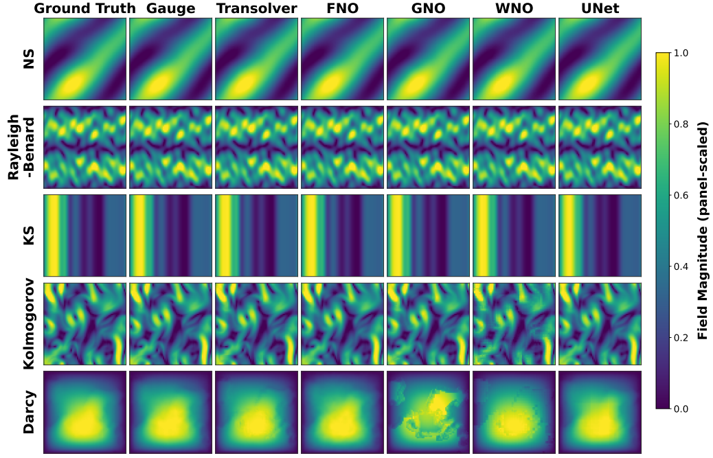
Figure 11: Representative native-resolution predictions. Columns compare the ground truth, GA-AMNO, Transolver, FNO, GNO, WNO, and UNet; rows correspond to Navier-Stokes, Rayleigh-Bénard, KS, Kolmogorov, and Darcy. Colors are independently scaled within each panel to emphasize spatial structure.
