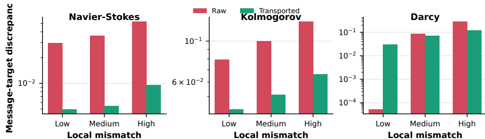
Figure 6: Source–target and transported-message–target discrepancy stratified by local geometric mismatch. The reduction measures message compatibility before aggregation, not the covariance defect of the learned connection.
