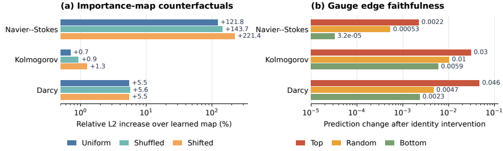
Figure 5: Causal tests of allocation and interaction readability. (a) Relative \ell_2 increase after replacing the learned importance map with uniform, shuffled, or shifted alternatives. (b) Prediction change after replacing transport with the identity on top-ranked, random, or bottom-ranked edge subsets.
