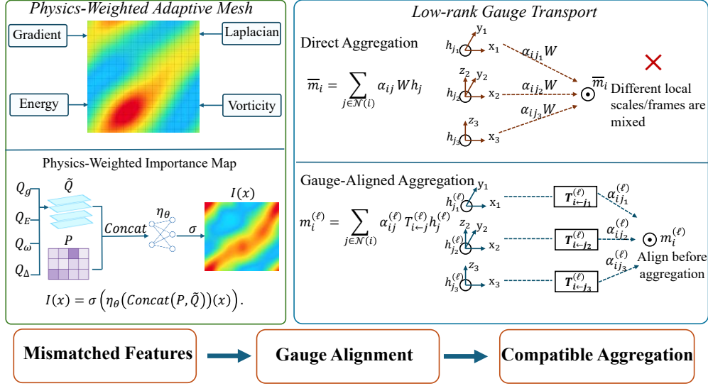
Figure 2: Conceptual overview of operator-readable adaptive computation. Physics-informed allocation explains where adaptive resolution is placed. The resulting nonuniform mesh produces unequal local discretization contexts, under which direct aggregation leaves the effects of geometric mismatch on cross-node interaction implicit. Gauge-aware transport instead maps each source feature into a target-conditioned representation before aggregation, making explicit how information is exchanged after the discretization changes.
