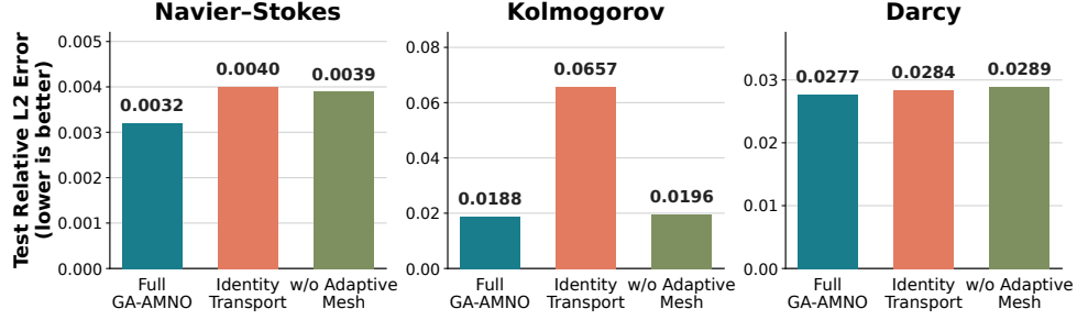
Figure 4: Ablation of the two core mechanisms. Identity Transport retains the adaptive mesh but removes learned representation transport, while w/o Adaptive Mesh retains the remaining solver without learned node relocation. Lower test relative \ell_2 error is better.
