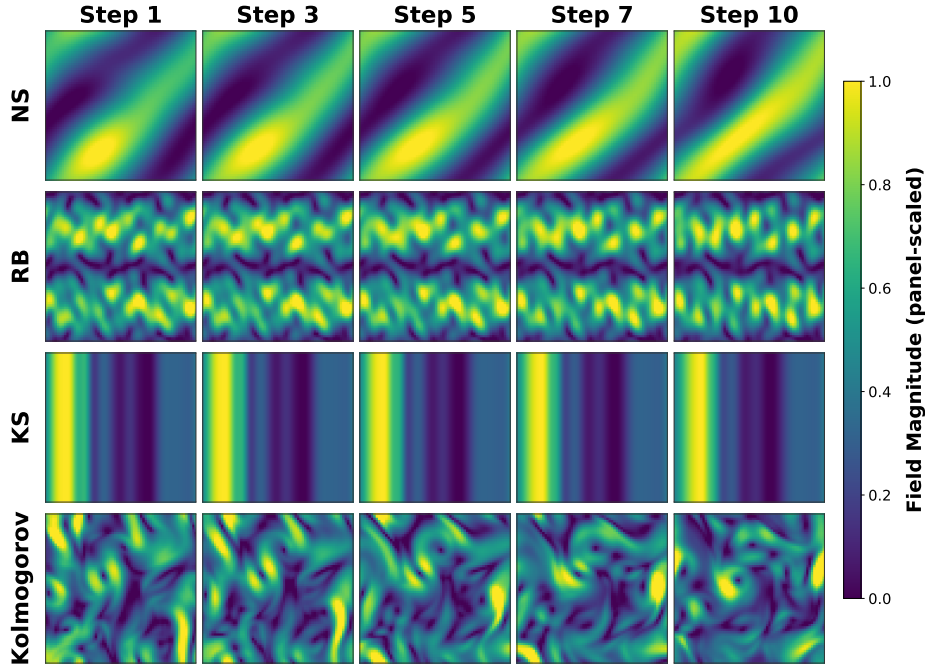
Figure 10: Selected GA-AMNO autoregressive predictions at rollout steps 1, 3, 5, 7, and 10 for Navier-Stokes, Rayleigh-Bénard, KS, and Kolmogorov. Colors are independently scaled within each panel, and the one-dimensional KS profile is repeated vertically for visualization.
