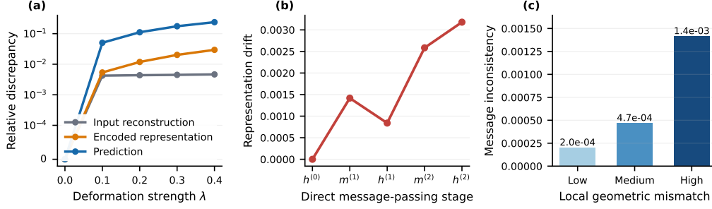
Figure 1: Preliminary diagnosis of the interaction effects induced by adaptive discretization on Navier-Stokes. (a) For the same physical state, increasing the topology-preserving deformation strength \lambda produces substantially larger representation and prediction discrepancies than input reconstruction discrepancy. (b) Representation drift emerges at direct aggregation and accumulates through subsequent message passing, where \mathbf{h}^{(\ell)} denotes the node representation at layer \ell and \mathbf{m}^{(\ell)} the aggregated message. (c) Message inconsistency increases with local geometric mismatch. Together, these results show that direct aggregation amplifies differences induced by unequal local discretization contexts.
