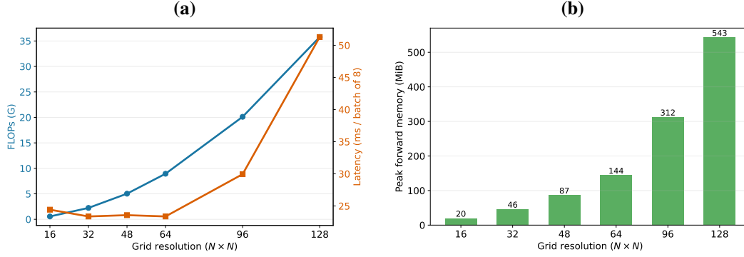
Figure 7: Computational scalability of GA-AMNO. (a) Counted FLOPs and synchronized forward latency at different grid resolutions. (b) Peak allocated forward memory. The same Navier-Stokes checkpoint and batch size 8 are used throughout.
