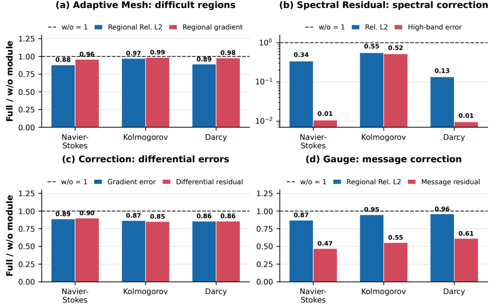
Figure 8: Targeted component ablations using frozen checkpoints. Each bar is the Full GA-AMNO metric divided by the corresponding w/o-module metric; lower is better and the dashed line denotes the ablated reference. Adaptive Mesh is evaluated in high-demand regions, Spectral Residual through field and high-band spectral errors, Differential Correction through gradient and differential errors, and Low-rank Gauge Transport through regional prediction and residual message–target discrepancy. Panel (b) uses a logarithmic vertical axis.
