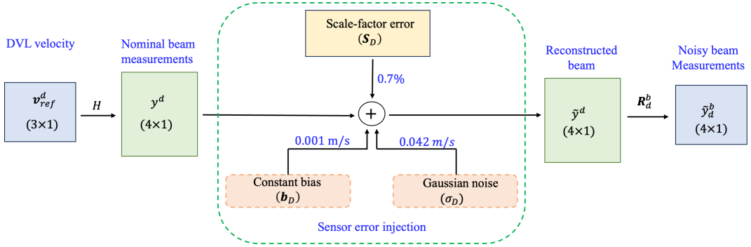
Figure 5: Pipeline for simulating noisy DVL beam measurements from the GT velocity.
