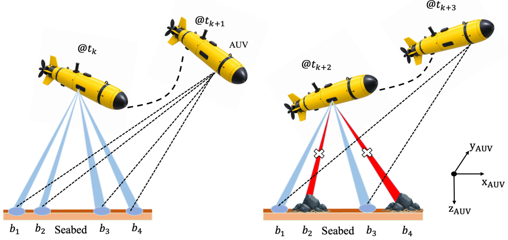
Figure 1: Illustration of an AUV maneuvering with a DVL under full and partial beam availability. The red beams indicate DVL measurements obstructed by underwater obstacles, while the remaining beams represent valid bottom-lock measurements during vehicle motion.
