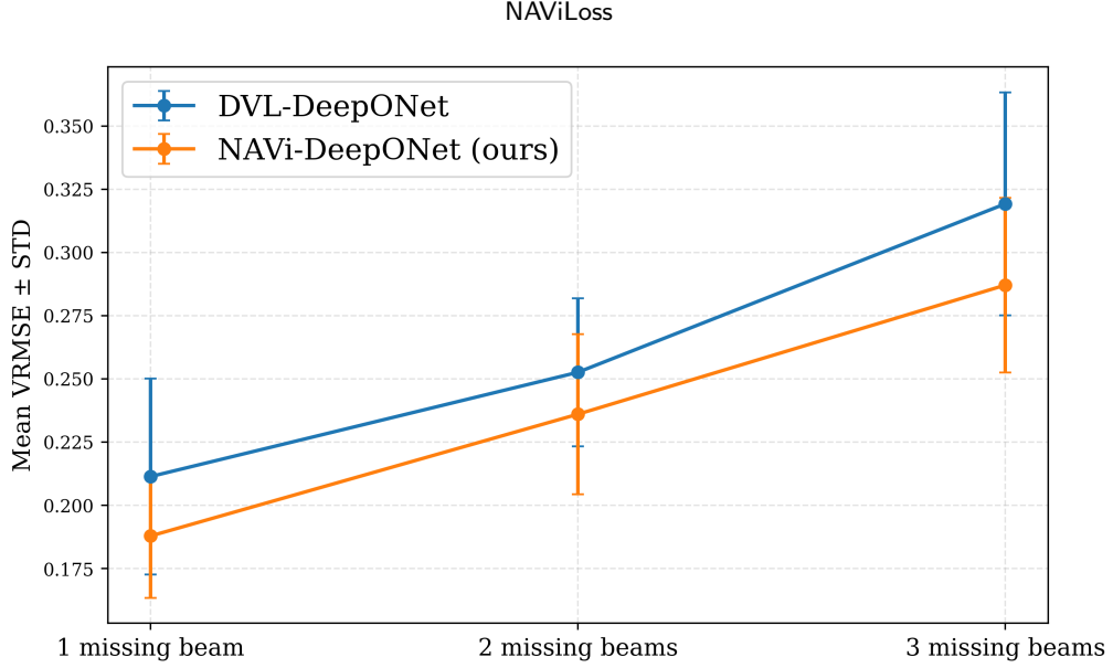
Figure 7: Velocity estimation performance under increasing DVL beam outages.
