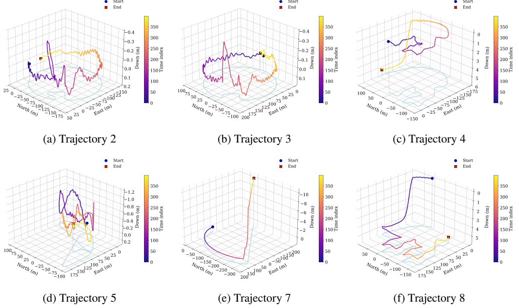
Figure 6: Three-dimensional GT paths of the test missions, with their corresponding North-East projections shown on the horizontal plane.
