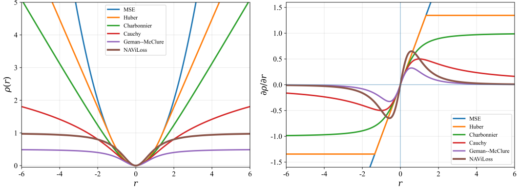
Figure 2: Comparison of NAViLoss with representative regression and robust loss functions. Left: penalty functions \rho(r) for residual r . Right: corresponding influence functions.
