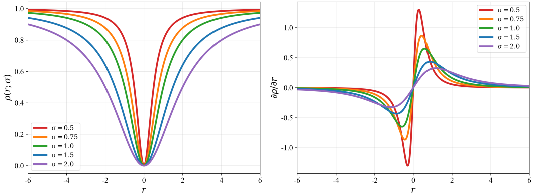
Figure 3: Effect of the uncertainty parameter \sigma on NAViLoss for fixed \lambda = 1 . Left: penalty function \rho(r; \sigma) for different uncertainty levels. Right: corresponding influence function.
